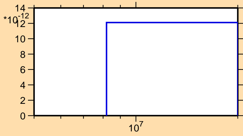
\sigma vs. E for ^{185}\text{Hg}(\text{mt } 34)
