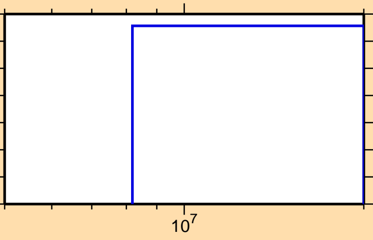
\sigma vs. E for ^{185}\text{Hg}(n,\text{pd})
