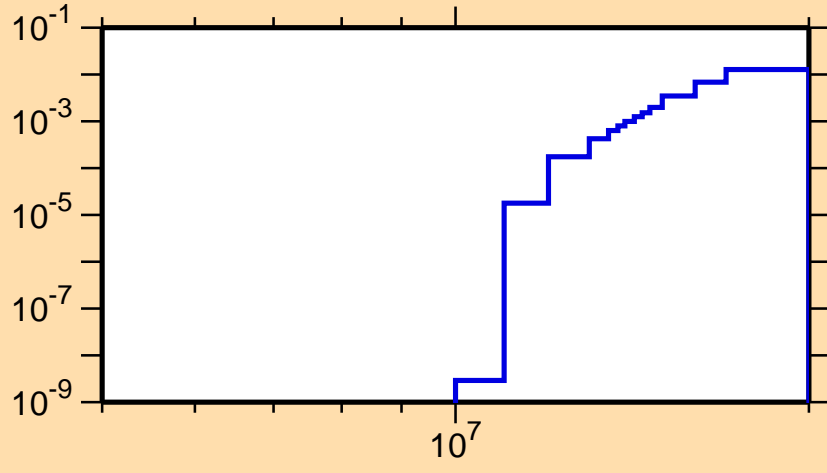
\sigma vs. E for ^{186}\text{Hg}(n,2n\alpha)
