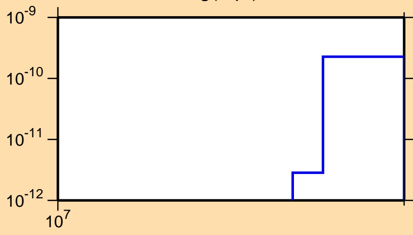
\sigma vs. E for ^{186}\text{Hg}(n,\text{pt})
