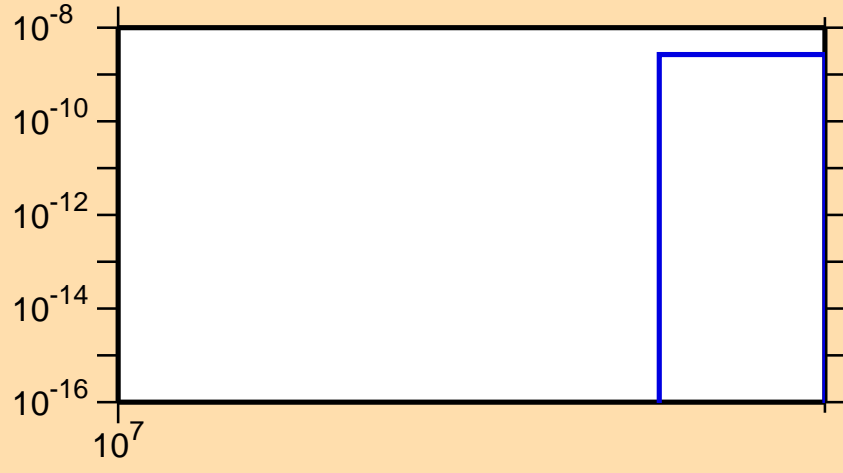
\sigma vs. E for ^{186}\text{Hg}(n,3n\alpha)
