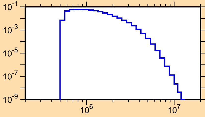
\sigma vs. E for ^{186}\text{Hg}(n,n_2)
