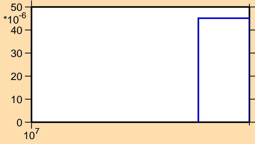
\sigma vs. E for ^{186}\text{Hg}(n,3n)
