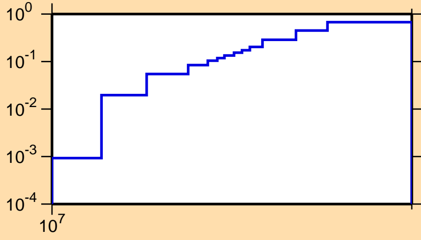
\sigma vs. E for ^{186}\text{Hg}(n,2n)
