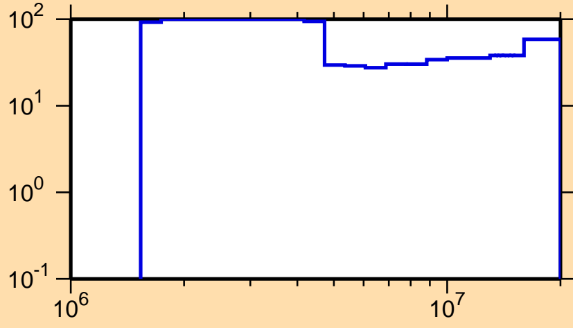
\Delta\sigma/\sigma vs. E for ^{186}\text{Hg}(n,n\text{cont.})
