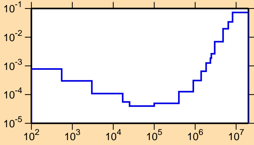
\sigma vs. E for ^{186}\text{Hg}(n,p)
