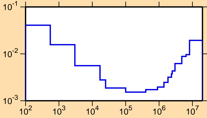
\sigma vs. E for ^{186}\text{Hg}(n,\alpha)
