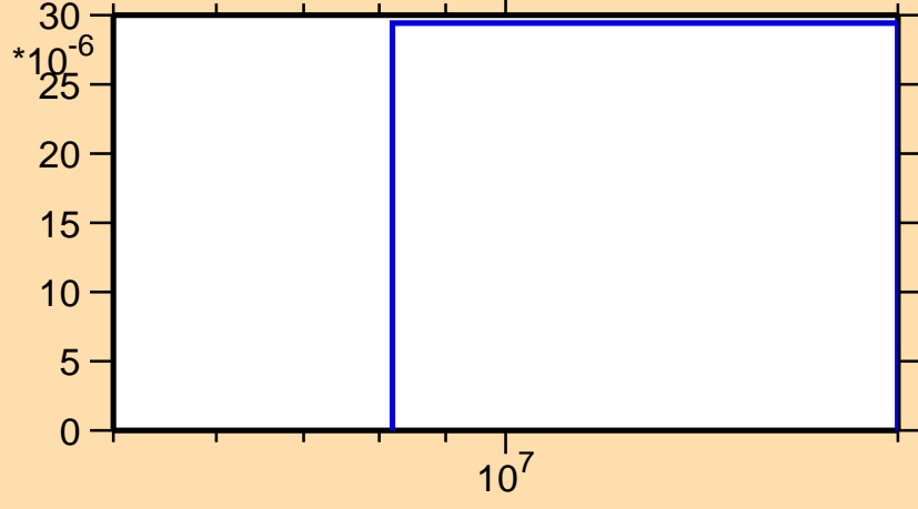
\sigma vs. E for ^{186}\text{Hg}(n,t)
