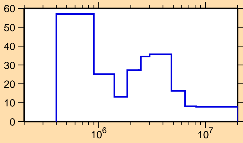
\Delta\sigma/\sigma vs. E for ^{186}\text{Hg}(n,\text{tot.})
