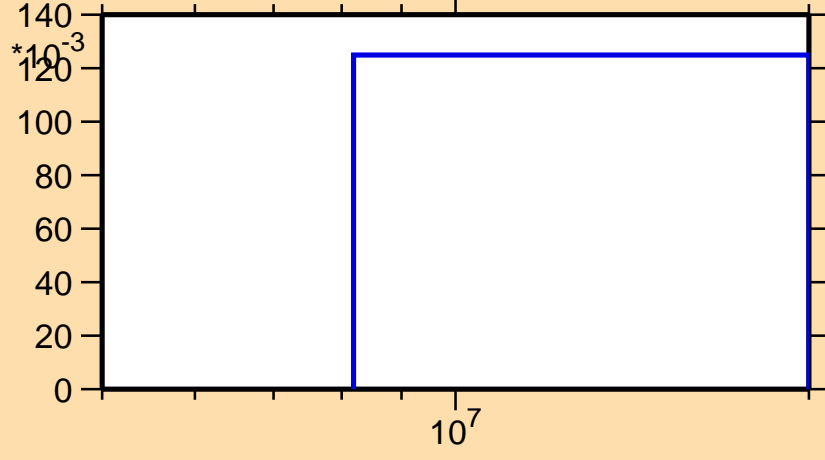
\sigma vs. E for ^{186}\text{Hg}(n,2n)
