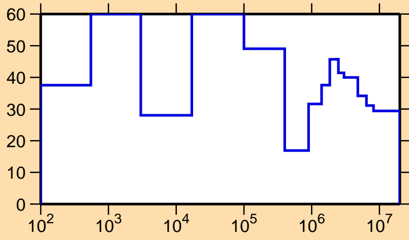
\Delta\sigma/\sigma vs. E for ^{186}\text{Hg}(n,\text{nonel.})
