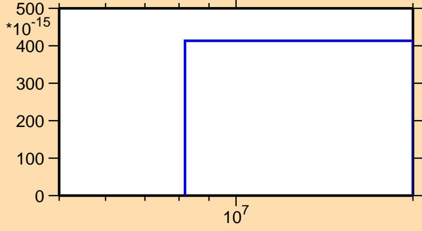
\sigma vs. E for ^{186}\text{Hg}(n,nt)
