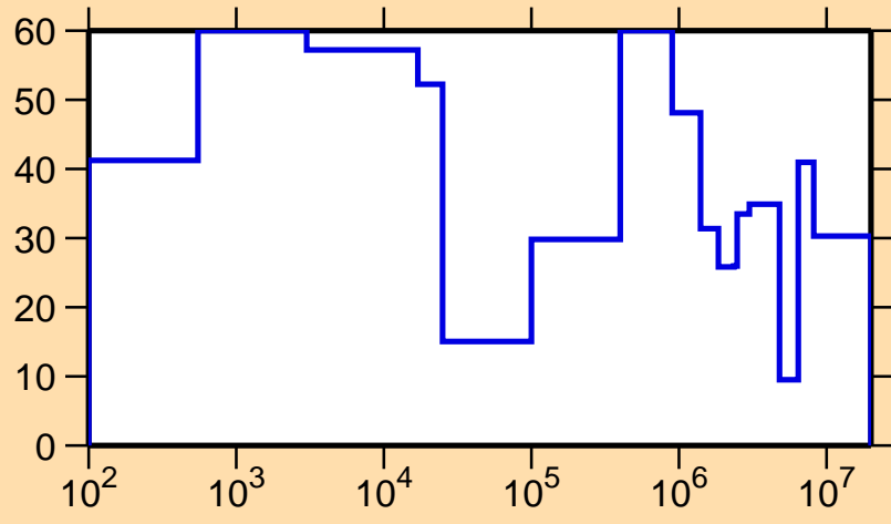
\Delta\sigma/\sigma vs. E for ^{186}\text{Hg}(n,\text{el.})
