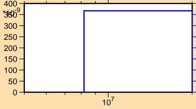
\sigma vs. E for ^{186}\text{Hg}(n,3n)
