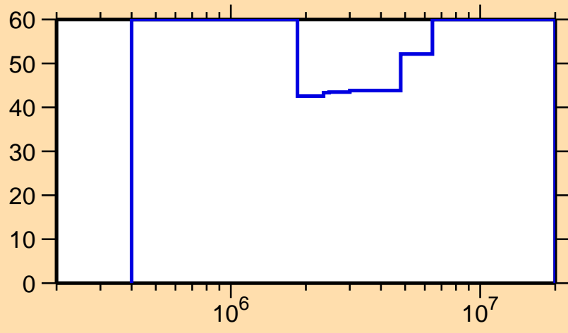
\Delta\sigma/\sigma vs. E for ^{186}\text{Hg}(n,n_1)
