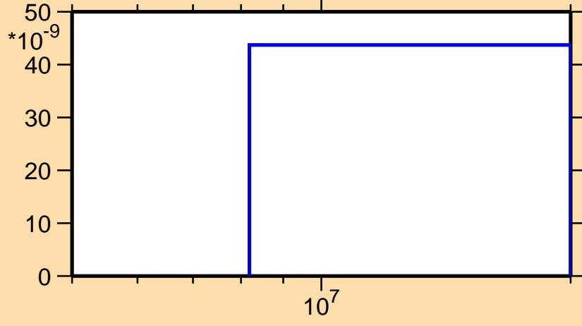
\sigma vs. E for ^{186}\text{Hg}(n,2np)
