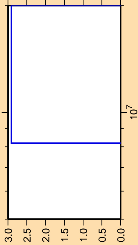
\Delta\sigma/\sigma vs. E for ^{186}\text{Hg}(n,nt)
