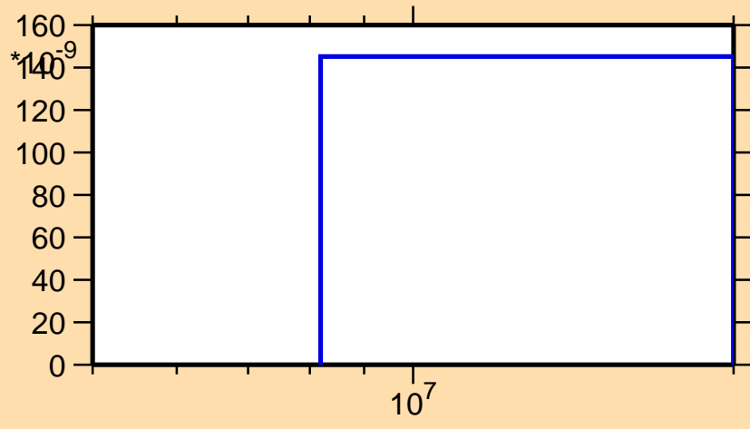
\sigma vs. E for ^{186}\text{Hg}(n,\text{He}3)
