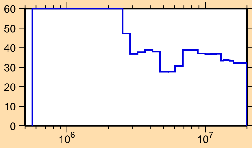
\Delta\sigma/\sigma vs. E for ^{187}\text{Hg}(n,n_1)
