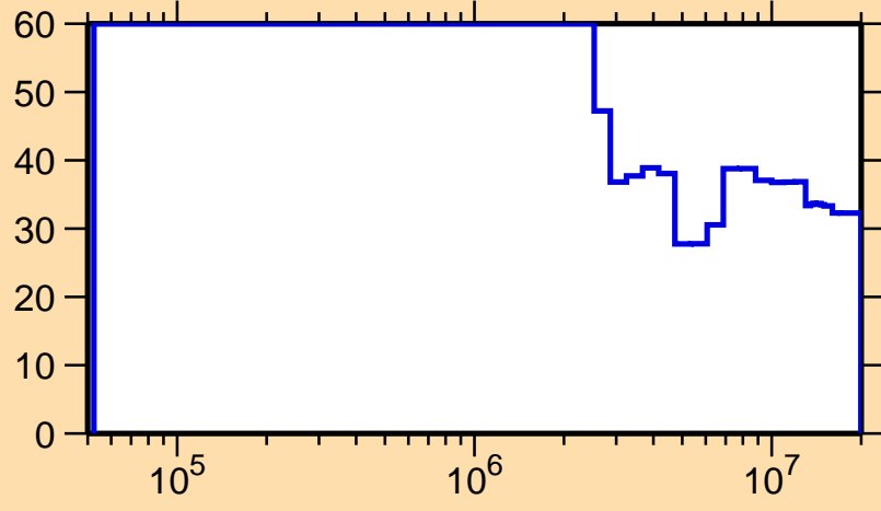
\Delta\sigma/\sigma vs. E for ^{187}\text{Hg}(n,n_1)
