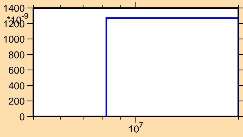
\sigma vs. E for ^{187}\text{Hg}(n,3n)
