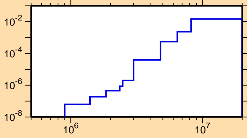
\sigma vs. E for ^{187}\text{Hg}(n,n\alpha)
