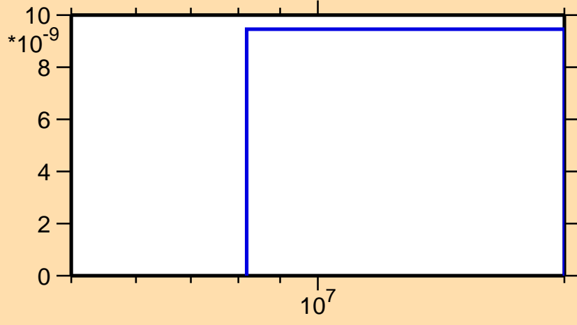
\sigma vs. E for ^{187}\text{Hg}(n,3n\alpha)
