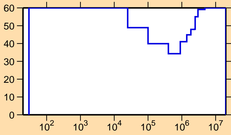
\Delta\sigma/\sigma vs. E for ^{187}\text{Hg}(n,\gamma)
