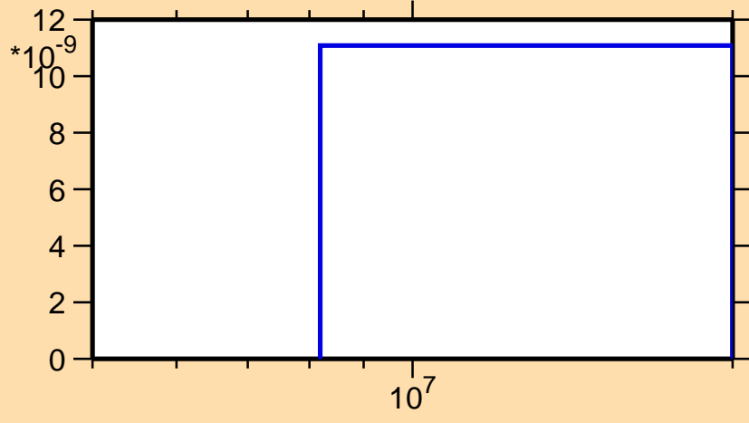
\sigma vs. E for ^{187}\text{Hg}(\text{mt117})
