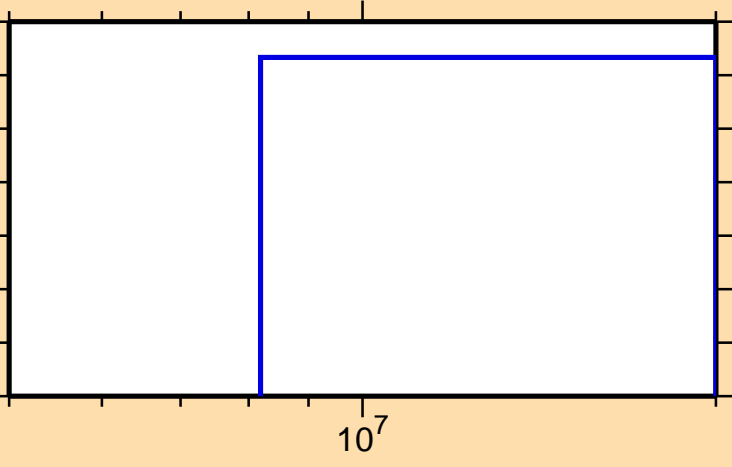
\sigma vs. E for ^{187}\text{Hg} (mt 45)
