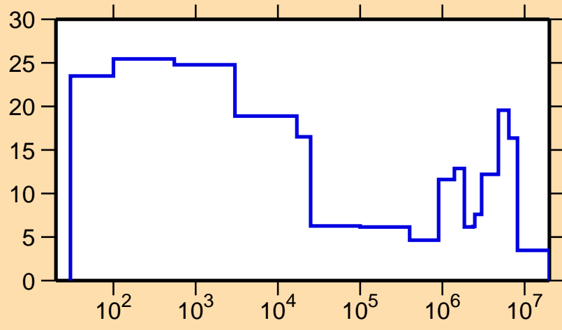
\Delta\sigma/\sigma vs. E for ^{187}\text{Hg}(n,\text{el.})
