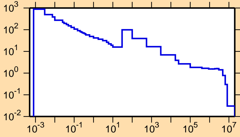
\sigma vs. E for ^{187}\text{Hg}(n,\gamma)
