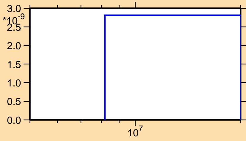
\sigma vs. E for ^{187}\text{Hg}(n,\text{pd})
