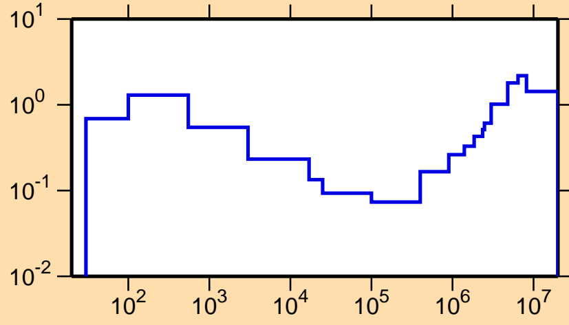
\sigma vs. E for ^{187}\text{Hg}(n,\text{inel.})
