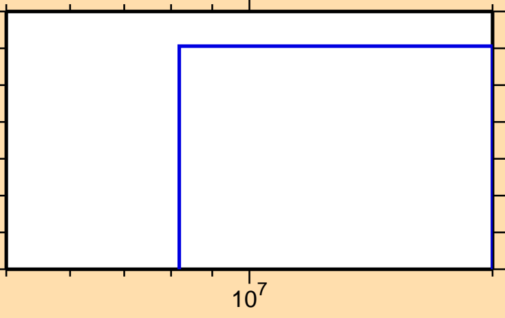
\sigma vs. E for ^{187}\text{Hg}(\text{mt117})
