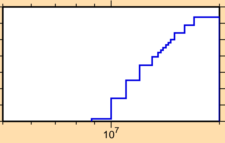
\sigma vs. E for ^{188}\text{Hg}(\text{mt117})
