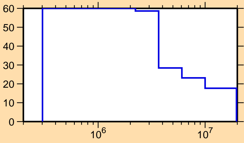
\Delta\sigma/\sigma vs. E for ^{188}\text{Hg}(n,n_1)
