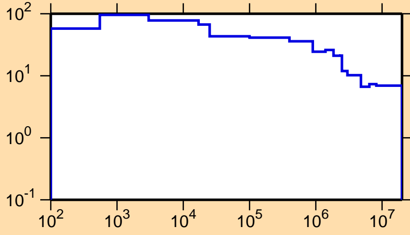
\Delta\sigma/\sigma vs. E for ^{188}\text{Hg}(n,\text{nonel.})
