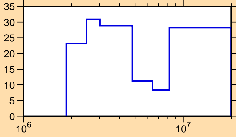
\Delta\sigma/\sigma vs. E for ^{188}\text{Hg}(n,n\text{cont.})
