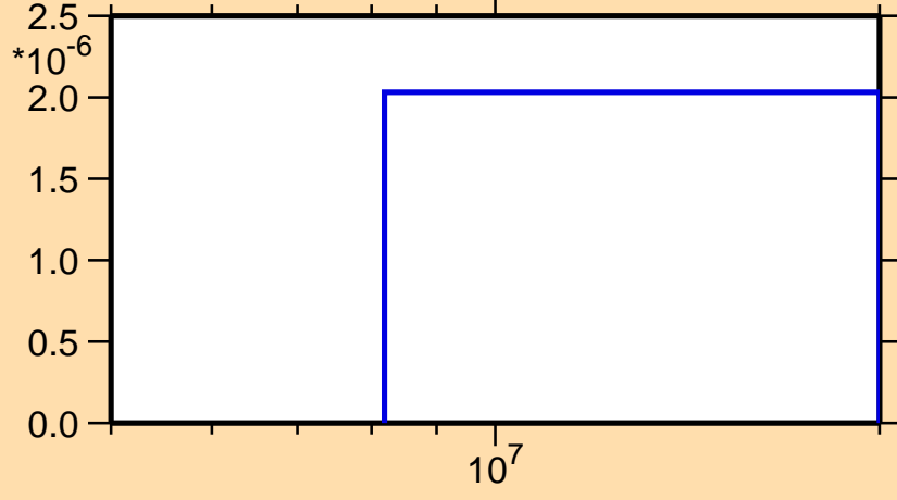
\sigma vs. E for ^{188}\text{Hg}(n,3n)
