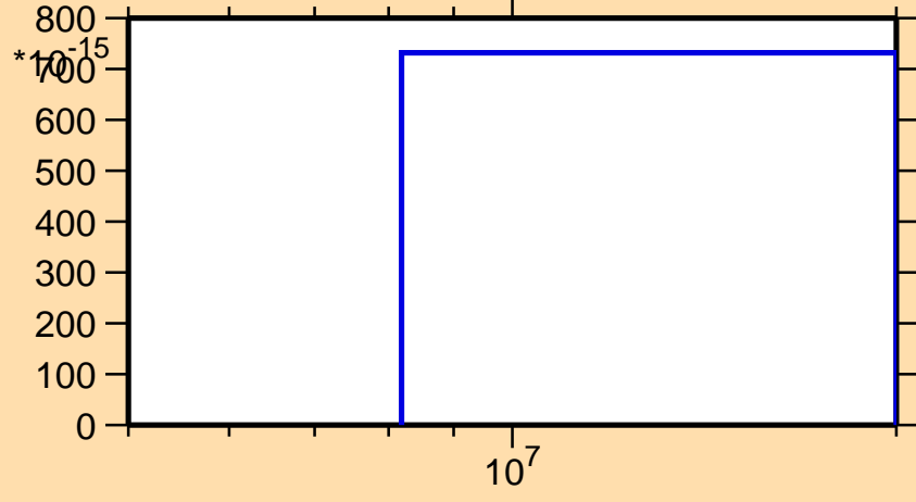
\sigma vs. E for ^{188}\text{Hg}(n,nt)
