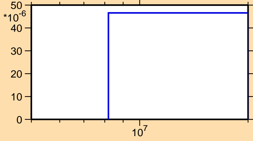
\sigma vs. E for ^{188}\text{Hg}(n,2n\alpha)
