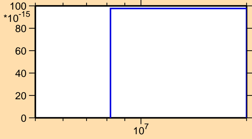
\sigma vs. E for ^{188}\text{Hg}(n,\text{pt})
