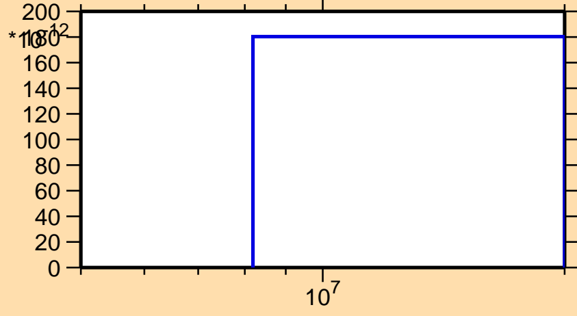
\sigma vs. E for ^{188}\text{Hg}(n,\text{nd})
