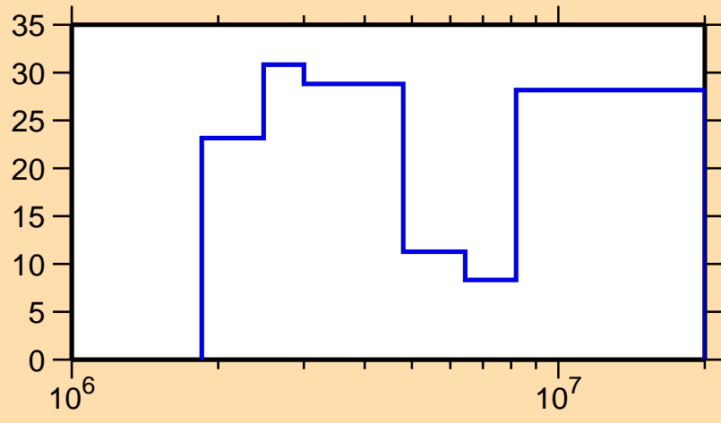
\Delta\sigma/\sigma vs. E for ^{188}\text{Hg}(n,n\text{cont.})
