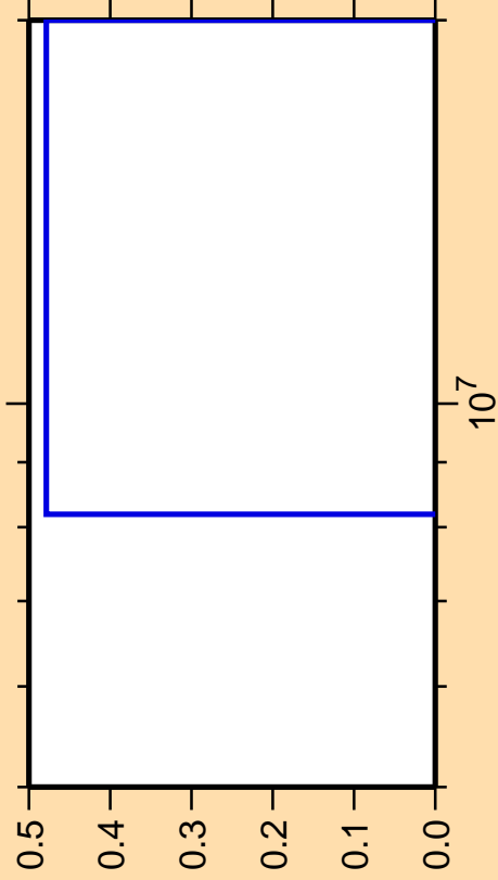
\Delta\sigma/\sigma vs. E for ^{188}\text{Hg}(n,\text{pt})
