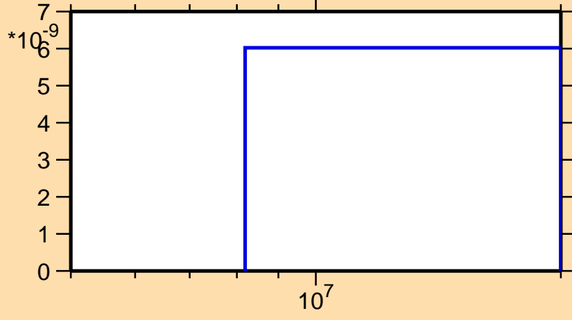
\sigma vs. E for ^{188}\text{Hg}(n,2np)
