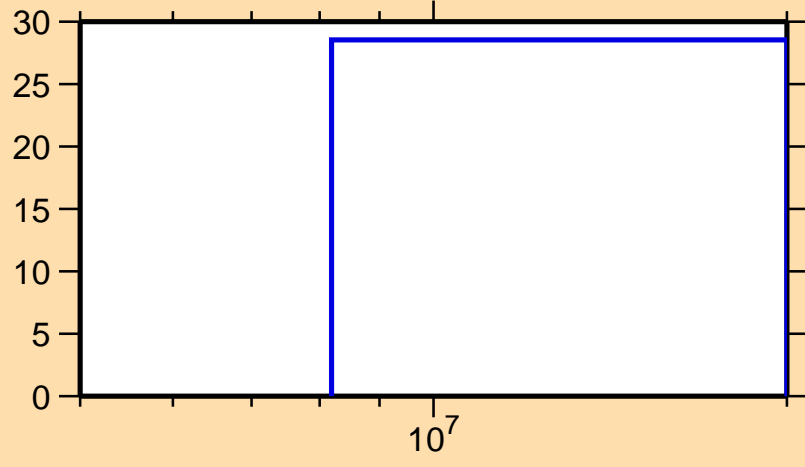
\Delta\sigma/\sigma vs. E for ^{188}\text{Hg}(n,\text{inel.})
