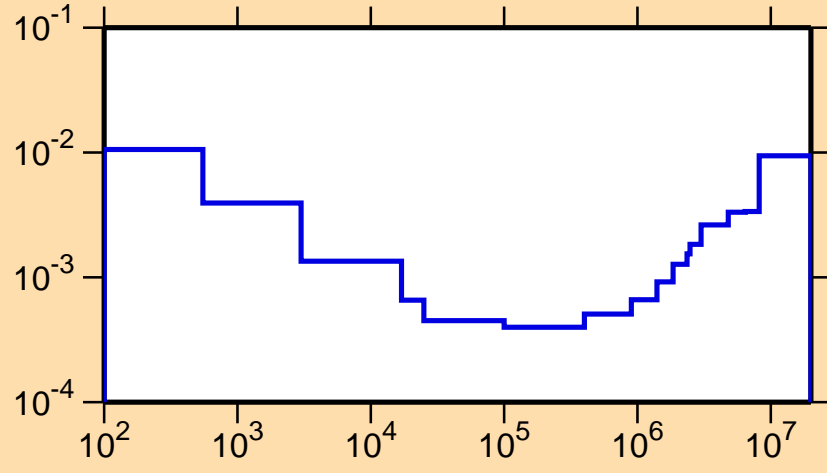
\sigma vs. E for ^{188}\text{Hg}(n,\alpha)
