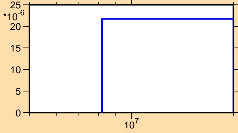
\sigma vs. E for ^{188}\text{Hg}(n,t)
