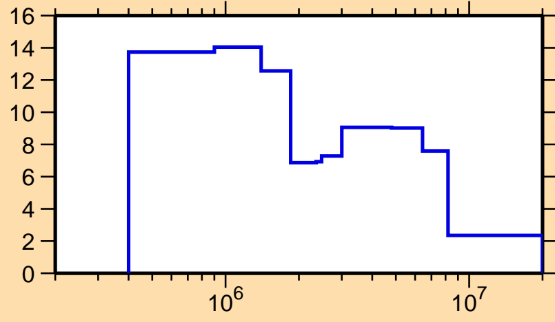
\Delta\sigma/\sigma vs. E for ^{188}\text{Hg}(n,\text{tot.})
