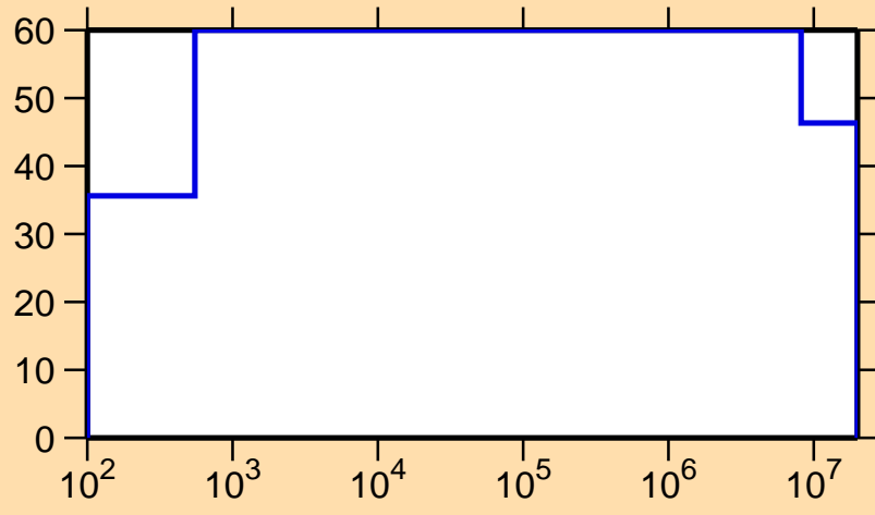
\Delta\sigma/\sigma vs. E for ^{188}\text{Hg}(n,p)
