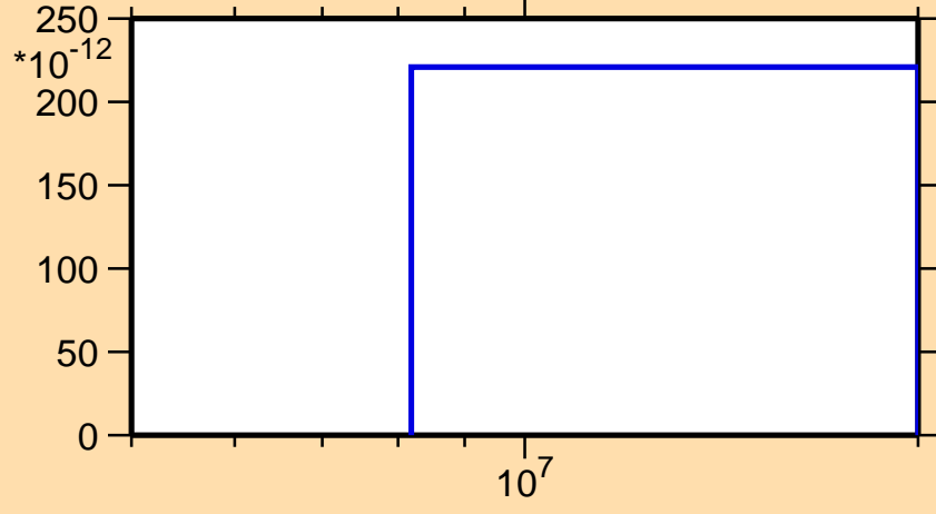
\sigma vs. E for ^{188}\text{Hg}(n,3n\alpha)
