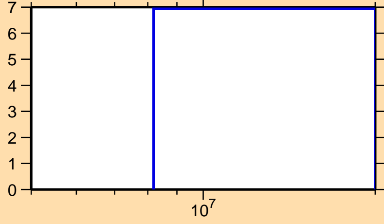
\Delta\sigma/\sigma vs. E for ^{188}\text{Hg}(n,\text{nonel.})
