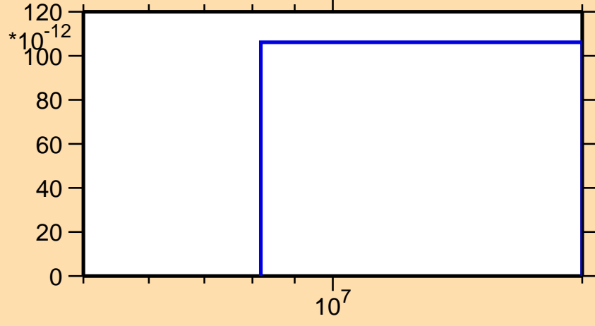
\sigma vs. E for ^{188}\text{Hg}(n,\text{pd})
