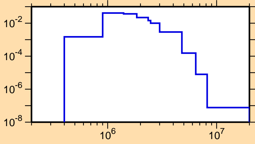
\sigma vs. E for ^{188}\text{Hg}(n,n_2)
