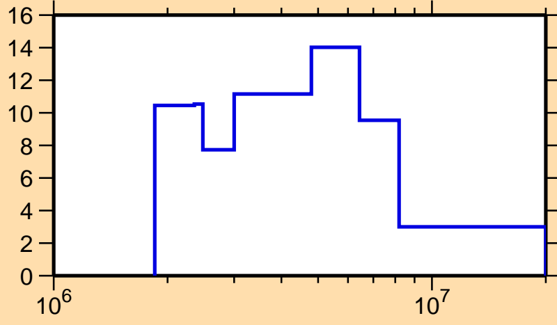
\Delta\sigma/\sigma vs. E for ^{188}\text{Hg}(n, \text{el.})
