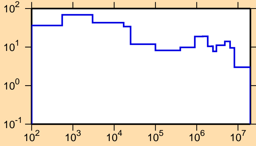
\Delta\sigma/\sigma vs. E for ^{188}\text{Hg}(n,\text{el.})
