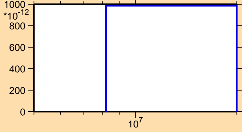
\sigma vs. E for ^{188}\text{Hg}(\text{mt117})
