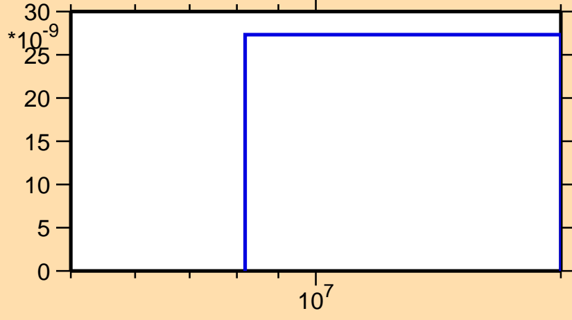
\sigma vs. E for ^{188}\text{Hg}(n,\text{He}3)
