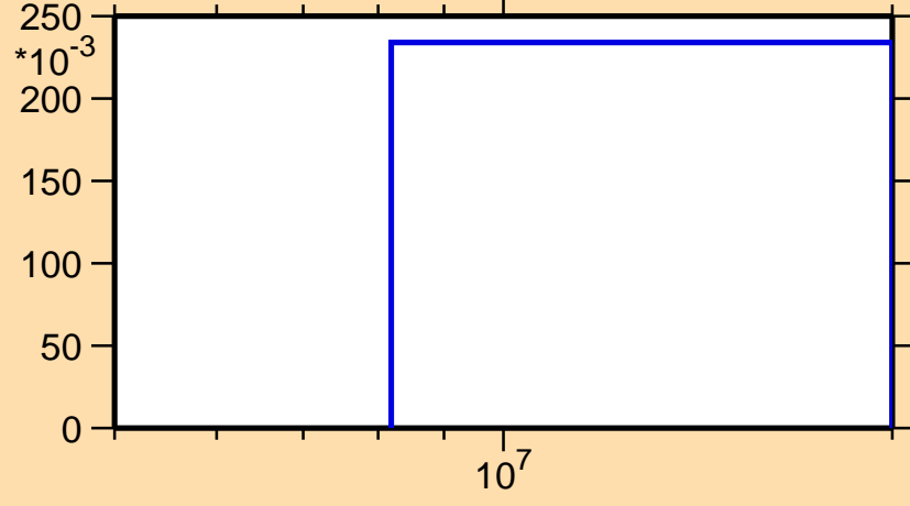
\sigma vs. E for ^{188}\text{Hg}(n,2n)
