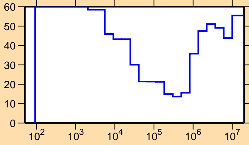
\Delta\sigma/\sigma vs. E for ^{189}\text{Hg}(n,\gamma)
