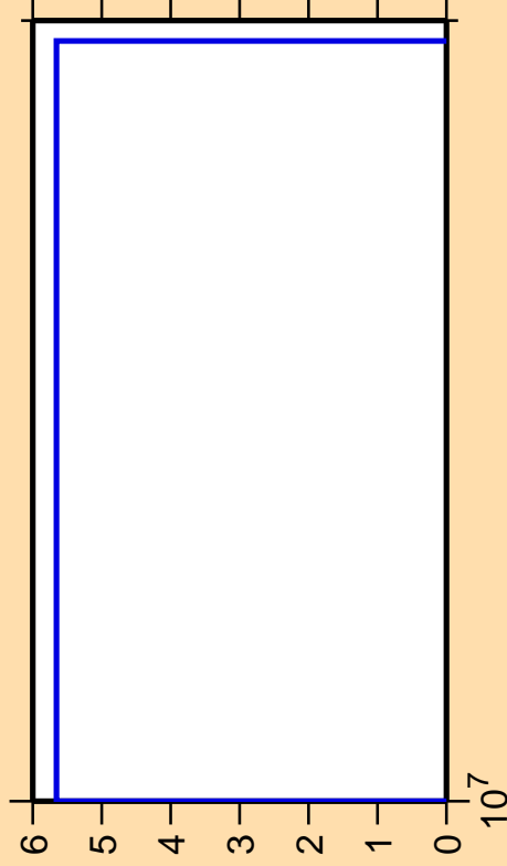
\Delta\sigma/\sigma vs. E for ^{189}\text{Hg}(n,nt)
