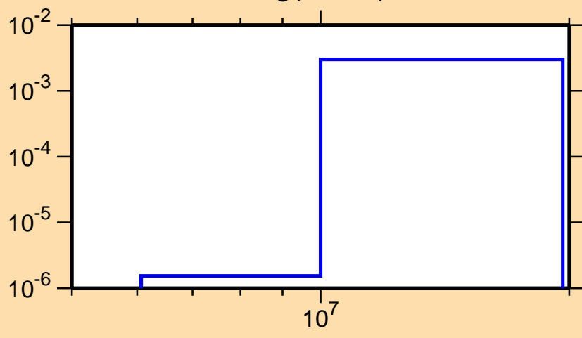
\sigma vs. E for ^{189}\text{Hg}(n,2n\alpha)
