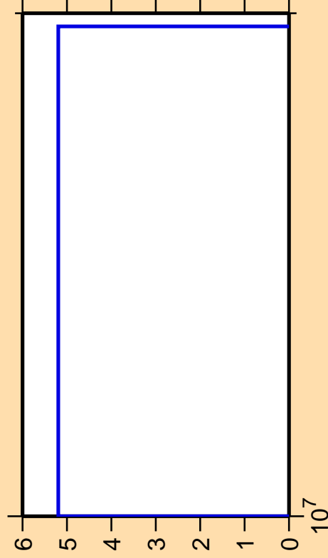
\Delta\sigma/\sigma vs. E for ^{189}\text{Hg} (mt 34)
