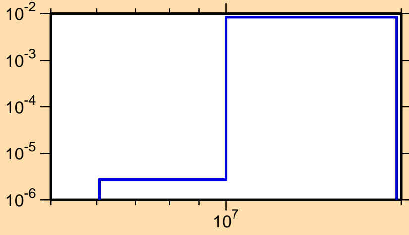
\sigma vs. E for ^{189}\text{Hg}(n,np)
