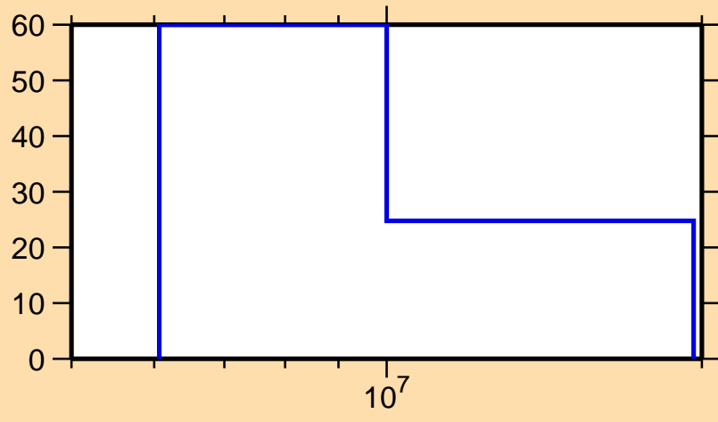
\Delta\sigma/\sigma vs. E for ^{189}\text{Hg}(n,2n)
