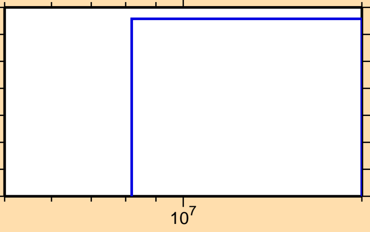
\sigma vs. E for ^{189}\text{Hg}(n,2np)
