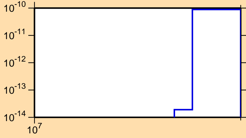
\sigma vs. E for ^{189}\text{Hg}(n,nt)
