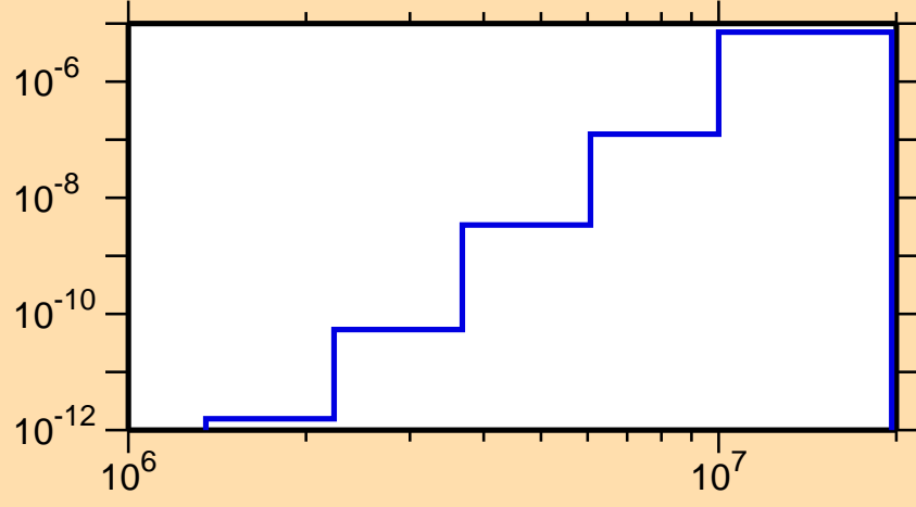
\sigma vs. E for ^{189}\text{Hg}(n,p\alpha)
