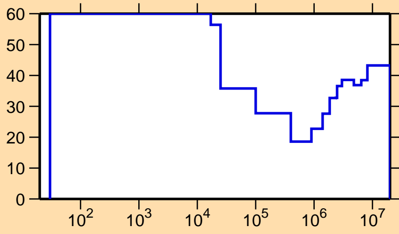
\Delta\sigma/\sigma vs. E for ^{189}\text{Hg}(n,\gamma)
