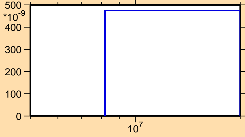
\sigma vs. E for ^{189}\text{Hg}(n,2np)
