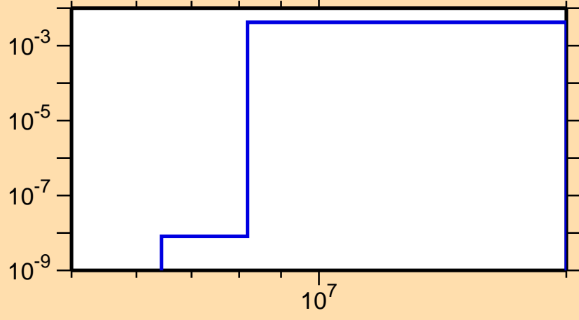
\sigma vs. E for ^{189}\text{Hg}(n,np)
