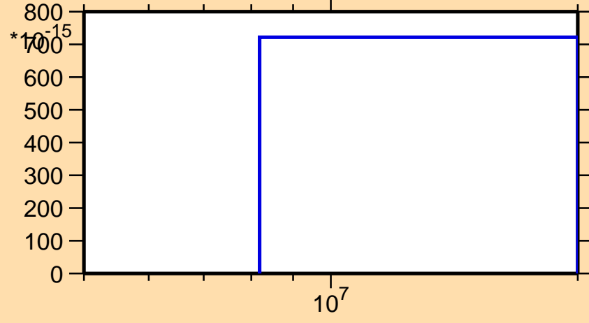
\sigma vs. E for ^{189}\text{Hg}(n,nt)
