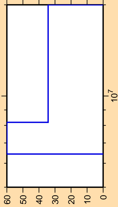
\Delta\sigma/\sigma vs. E for ^{189}\text{Hg}(n,2n)
