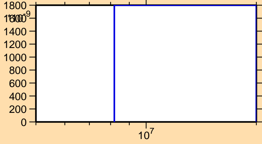
\sigma vs. E for ^{189}\text{Hg}(n,3n)
