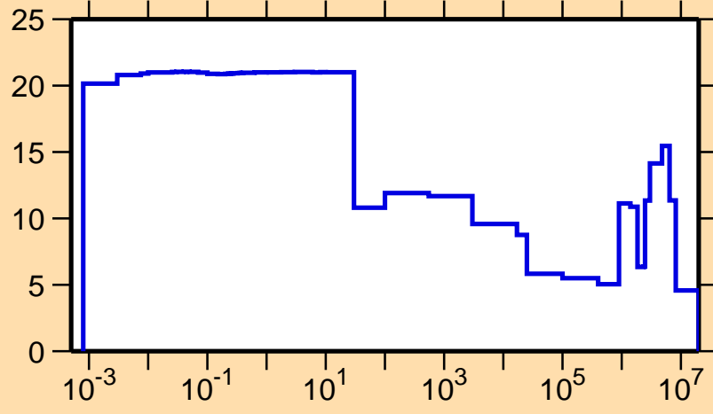
\Delta\sigma/\sigma vs. E for ^{189}\text{Hg}(n,\text{el.})
