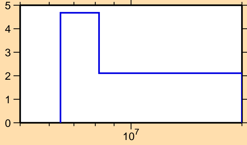
\Delta\sigma/\sigma vs. E for ^{189}\text{Hg}(n,\text{tot.})
