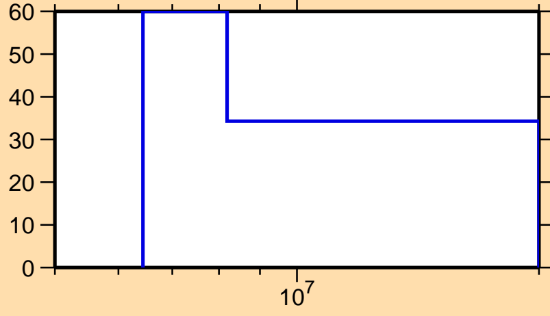
\Delta\sigma/\sigma vs. E for ^{189}\text{Hg}(n,2n)
