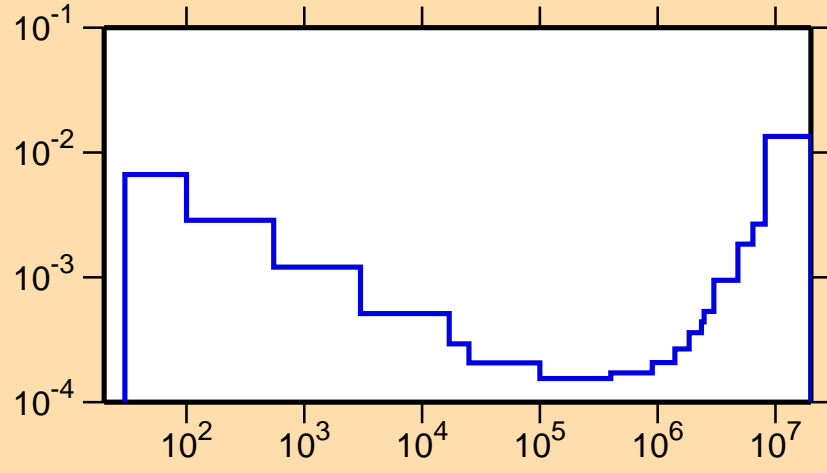
\sigma vs. E for ^{189}\text{Hg}(n,\alpha)
