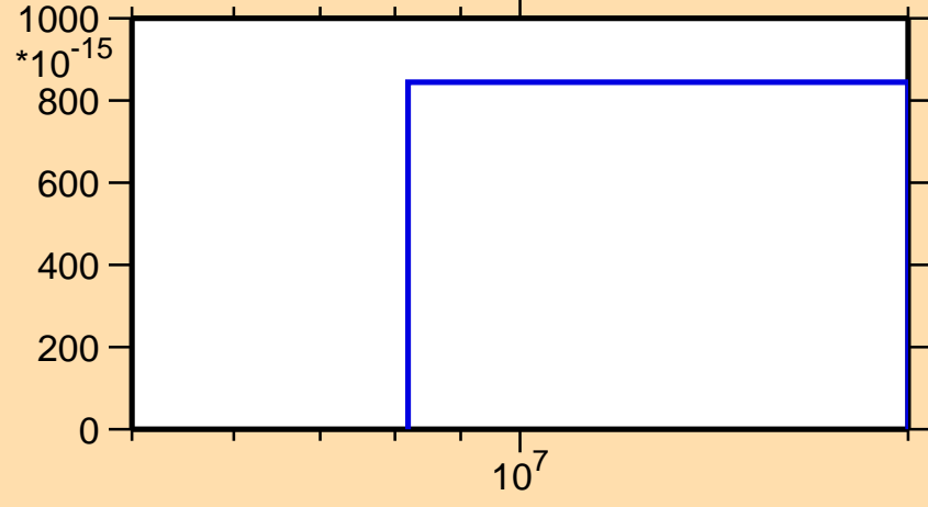
\sigma vs. E for ^{189}\text{Hg} (mt 34)
