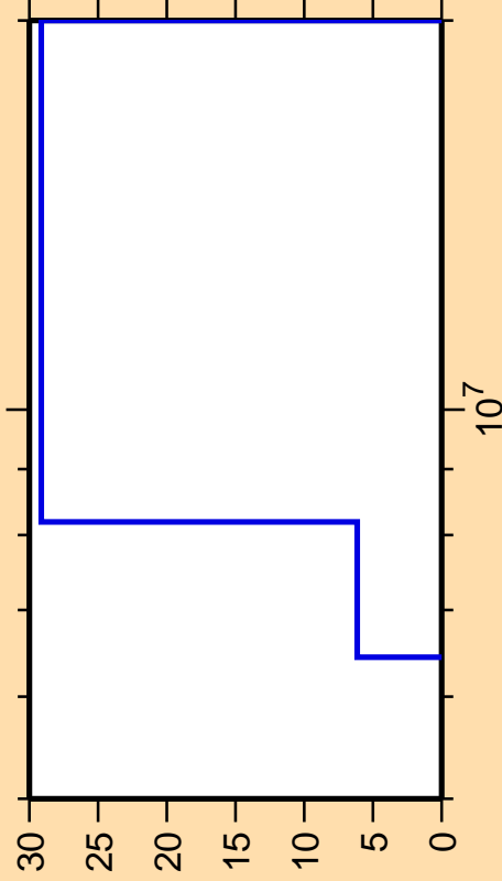
\Delta\sigma/\sigma vs. E for ^{189}\text{Hg}(n,n\text{cont.})
