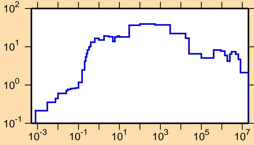
\Delta\sigma/\sigma vs. E for ^{189}\text{Hg}(n,\text{tot.})
