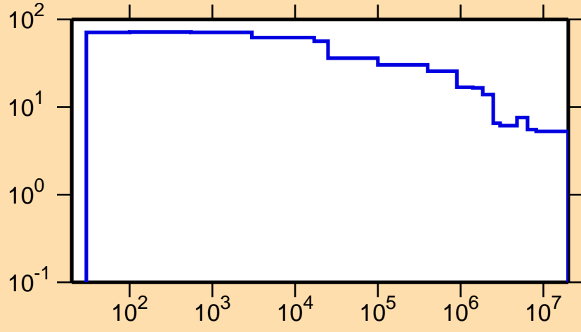
\Delta\sigma/\sigma vs. E for ^{189}\text{Hg}(n,\text{nonel.})
