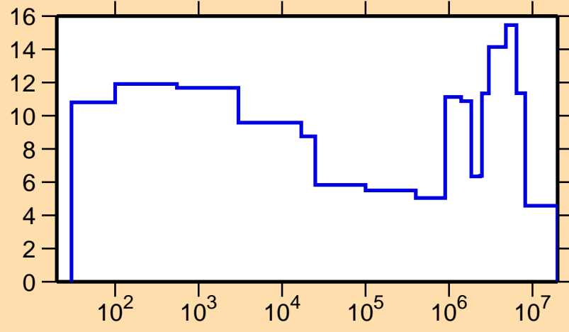
\Delta\sigma/\sigma vs. E for ^{189}\text{Hg}(n,\text{el.})
