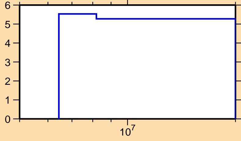
\Delta\sigma/\sigma vs. E for ^{189}\text{Hg}(n,\text{nonel.})
