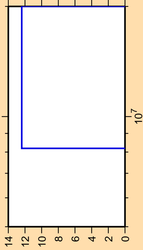
\Delta\sigma/\sigma vs. E for ^{189}\text{Hg}(n,\text{pt})
