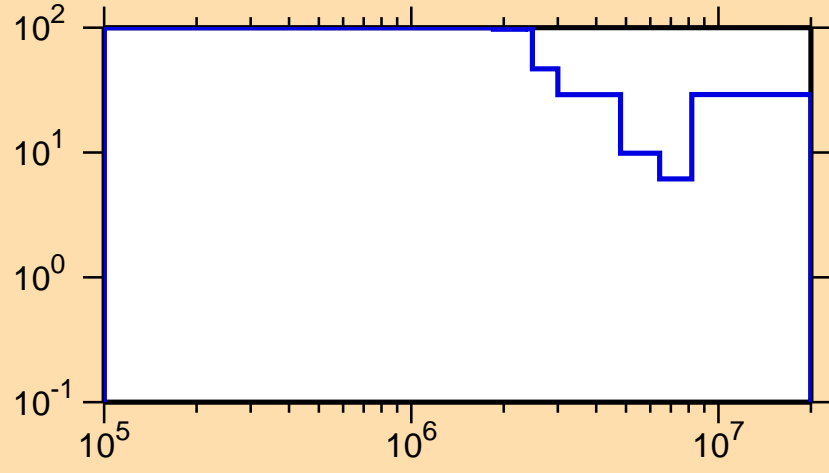
\Delta\sigma/\sigma vs. E for ^{189}\text{Hg}(n,n\text{cont.})
