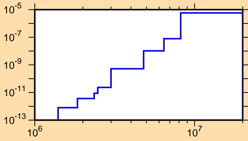
\sigma vs. E for ^{189}\text{Hg}(n,p\alpha)
