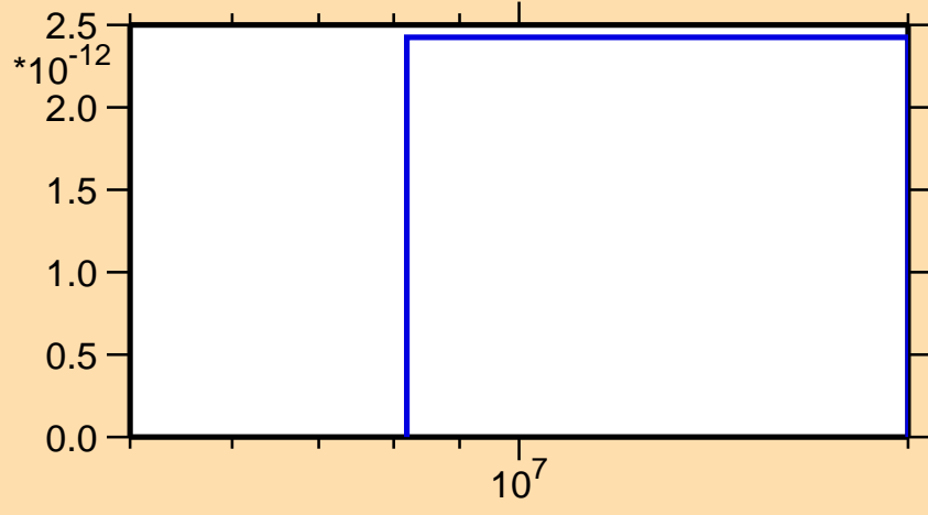
\sigma vs. E for ^{189}\text{Hg}(n,\text{pt})
