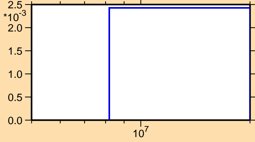
\sigma vs. E for ^{189}\text{Hg}(n,2n\alpha)
