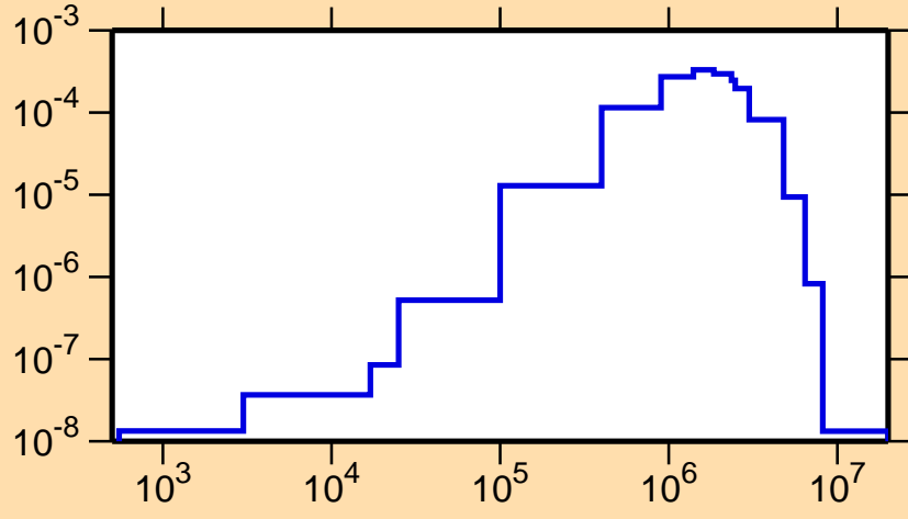
\sigma vs. E for ^{189}\text{Hg}(n,n_1)
