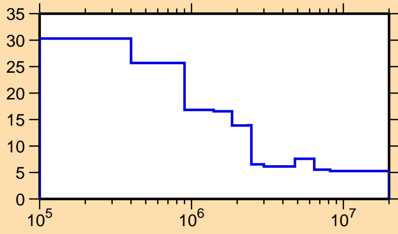
\Delta\sigma/\sigma vs. E for ^{189}\text{Hg}(n,\text{nonel.})
