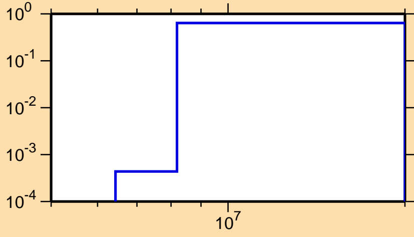
\sigma vs. E for ^{189}\text{Hg}(n,2n)
