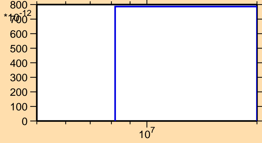
\sigma vs. E for ^{189}\text{Hg}(\text{mt117})
