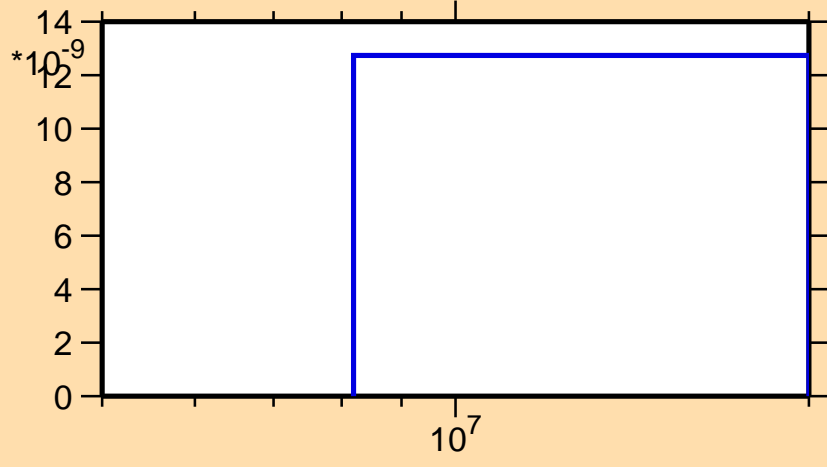
\sigma vs. E for ^{189}\text{Hg} (mt 45)
