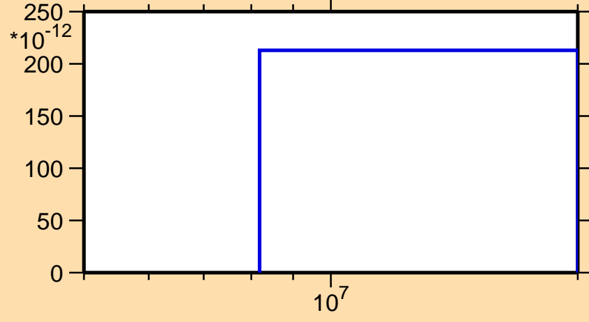
\sigma vs. E for ^{189}\text{Hg}(n,3n\alpha)
