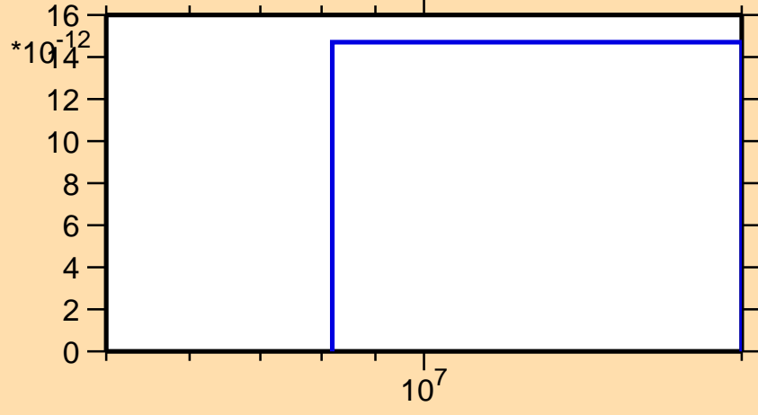
\sigma vs. E for ^{189}\text{Hg}(n,\text{pd})
