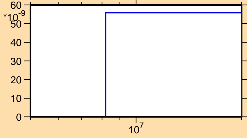
\sigma vs. E for ^{189}\text{Hg}(n,\text{He}3)
