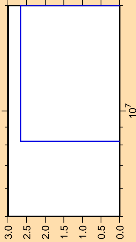
\Delta\sigma/\sigma vs. E for ^{189}\text{Hg} (mt 34)
