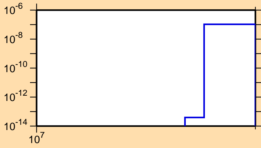
\sigma vs. E for ^{190}\text{Hg}(n,3n\alpha)
