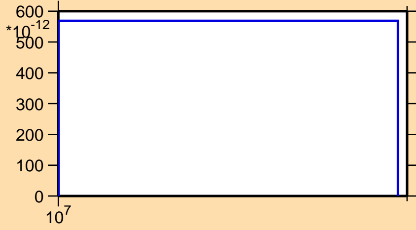
\sigma vs. E for ^{190}\text{Hg}(n,3n\alpha)
