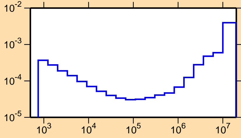
\sigma vs. E for ^{190}\text{Hg}(n,\alpha)
