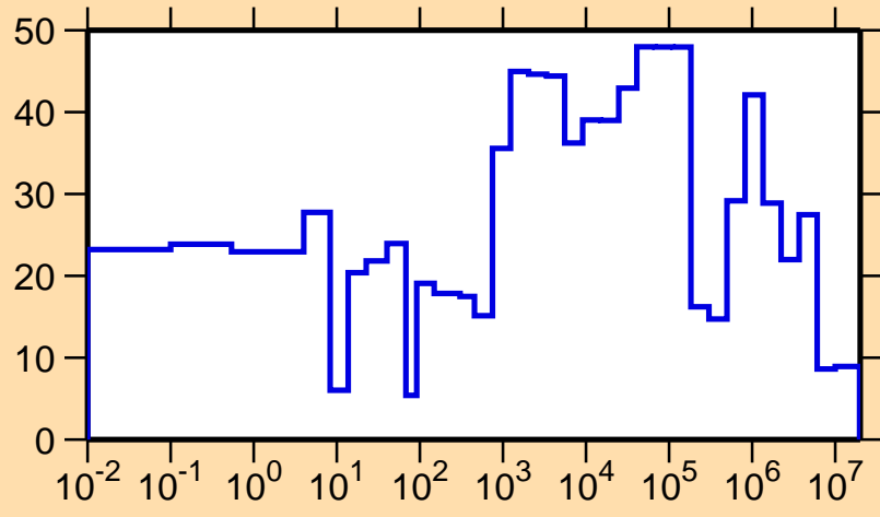
\Delta\sigma/\sigma vs. E for ^{190}\text{Hg}(n,\text{el.})
