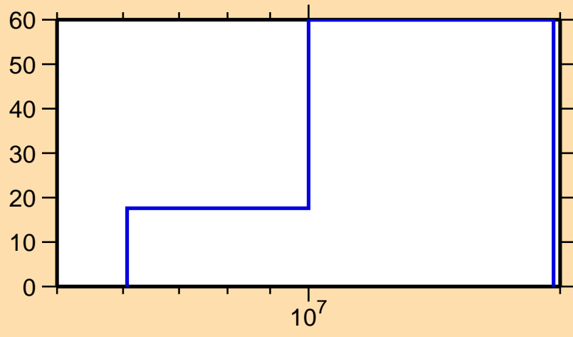
\Delta\sigma/\sigma vs. E for ^{190}\text{Hg}(n,\text{inel.})
