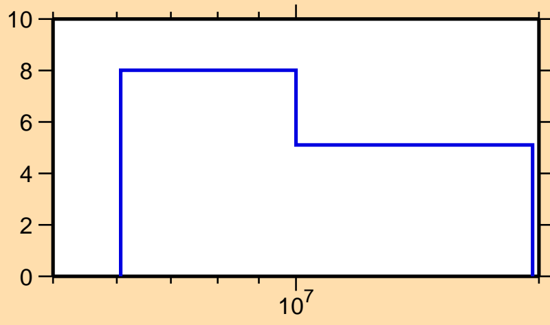
\Delta\sigma/\sigma vs. E for ^{190}\text{Hg}(n,\text{nonel.})
