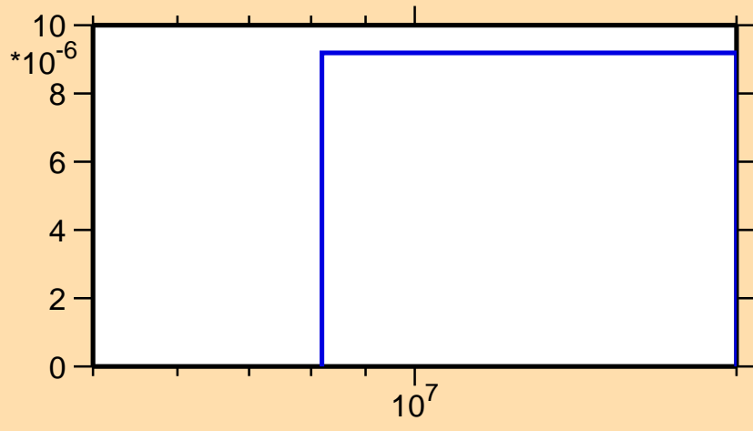
\sigma vs. E for ^{190}\text{Hg}(n,t)
