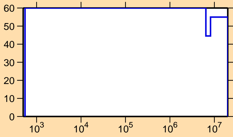
\Delta\sigma/\sigma vs. E for ^{190}\text{Hg}(n,p)
