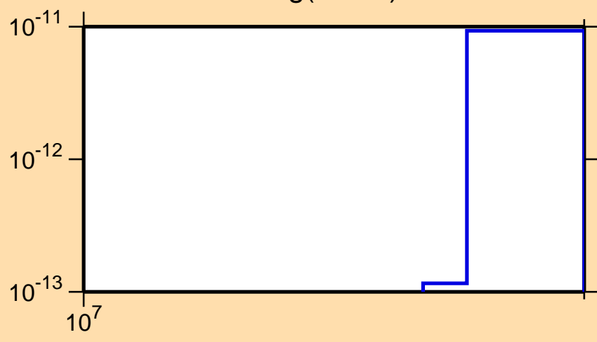
\sigma vs. E for ^{191}\text{Hg} (mt 34)
