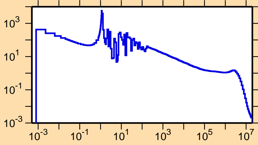
\sigma vs. E for ^{191}\text{Hg}(n,\gamma)
