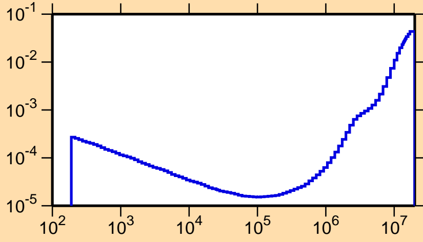
\sigma vs. E for ^{191}\text{Hg}(n,p)
