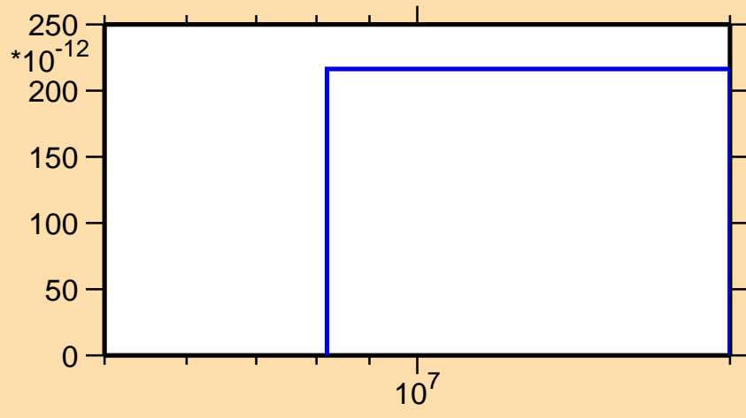
\sigma vs. E for ^{191}\text{Hg} (mt 45)
