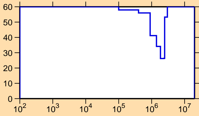
\Delta\sigma/\sigma vs. E for ^{191}\text{Hg}(n,\gamma)
