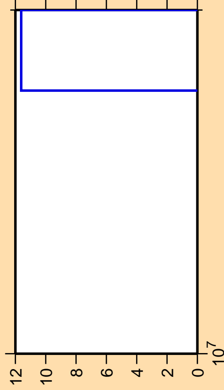
\Delta\sigma/\sigma vs. E for ^{191}\text{Hg}(n,3n\alpha)
