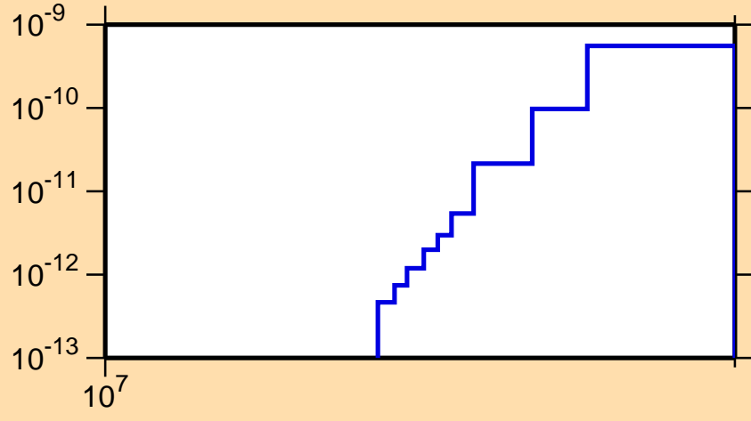
\sigma vs. E for ^{191}\text{Hg}(\text{mt117})
