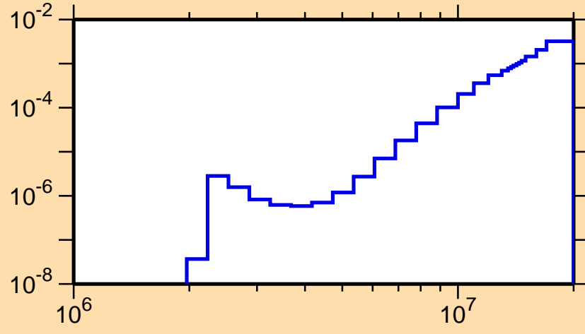
\sigma vs. E for ^{191}\text{Hg}(n,n\alpha)
