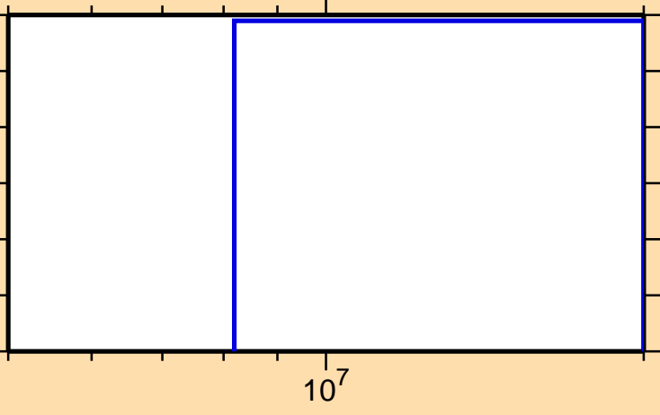
\sigma vs. E for ^{191}\text{Hg}(n,\text{nd})
