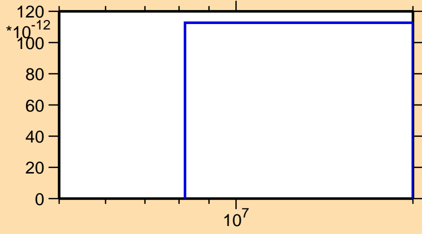
\sigma vs. E for ^{191}\text{Hg}(\text{mt } 45)
