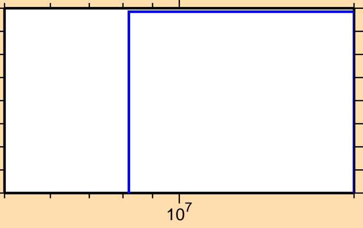
\sigma vs. E for ^{191}\text{Hg}(n,3n\alpha)
