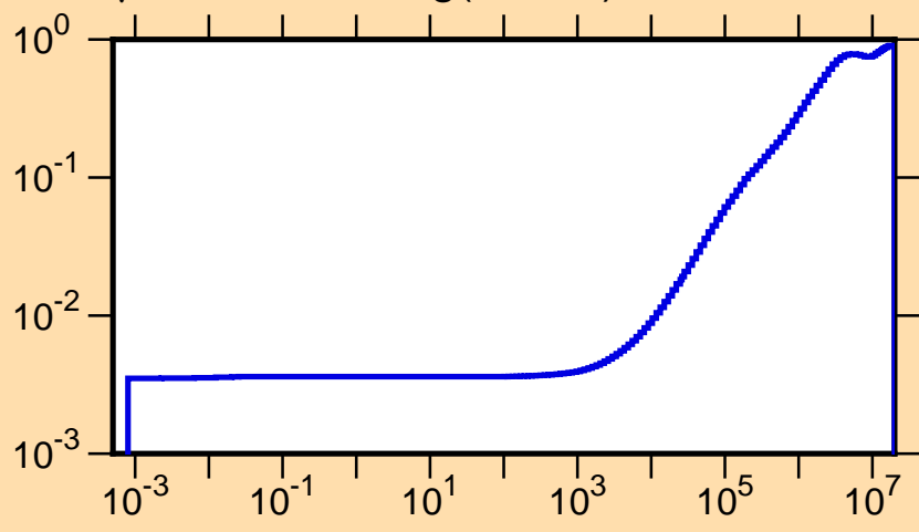
\mu vs. E for ^{192}\text{Hg}(\text{mt251})
