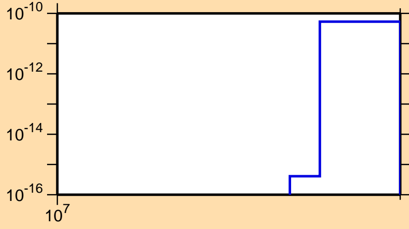
\sigma vs. E for ^{192}\text{Hg}(n,nt)
