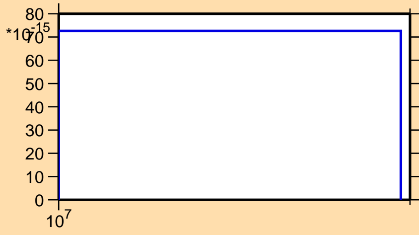
\sigma vs. E for ^{192}\text{Hg}(n,\text{pd})
