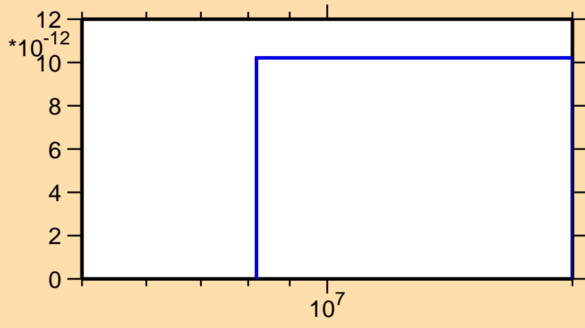
\sigma vs. E for ^{192}\text{Hg} (mt 45)
