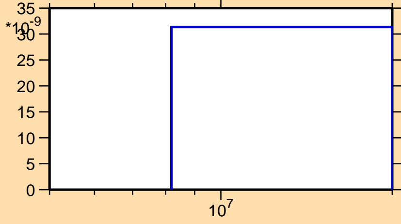
\sigma vs. E for ^{192}\text{Hg}(n,3n\alpha)
