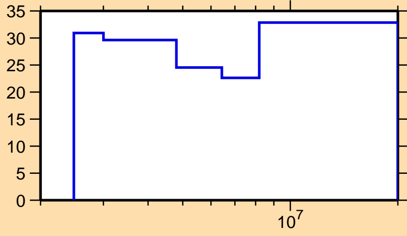
\Delta\sigma/\sigma vs. E for ^{192}\text{Hg}(n,n\text{cont.})
