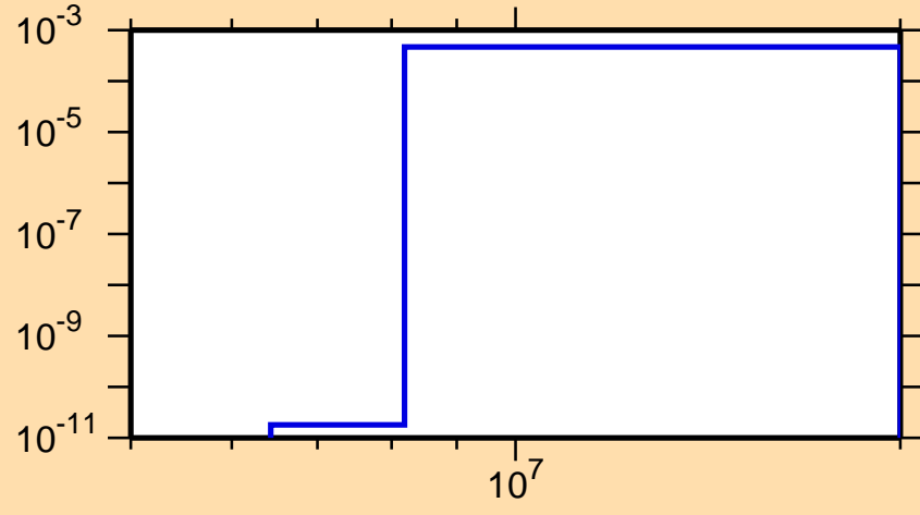
\sigma vs. E for ^{192}\text{Hg}(n,d)
