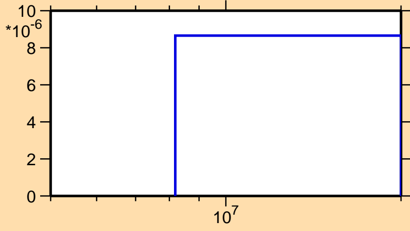
\sigma vs. E for ^{192}\text{Hg}(n,t)
