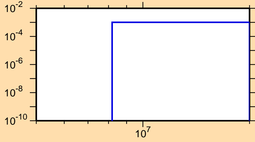
\sigma vs. E for ^{192}\text{Hg}(n,np)
