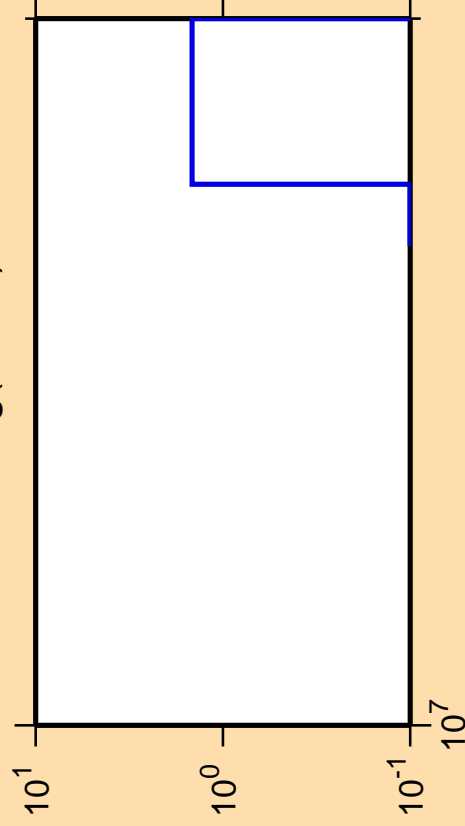
\Delta\sigma/\sigma vs. E for ^{193}\text{Hg}(n,3n\alpha)
