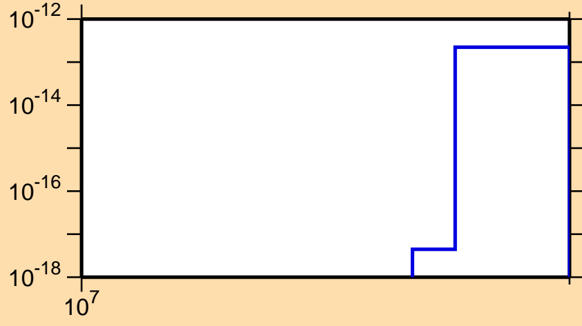
\sigma vs. E for ^{193}\text{Hg}(n,3n\alpha)
