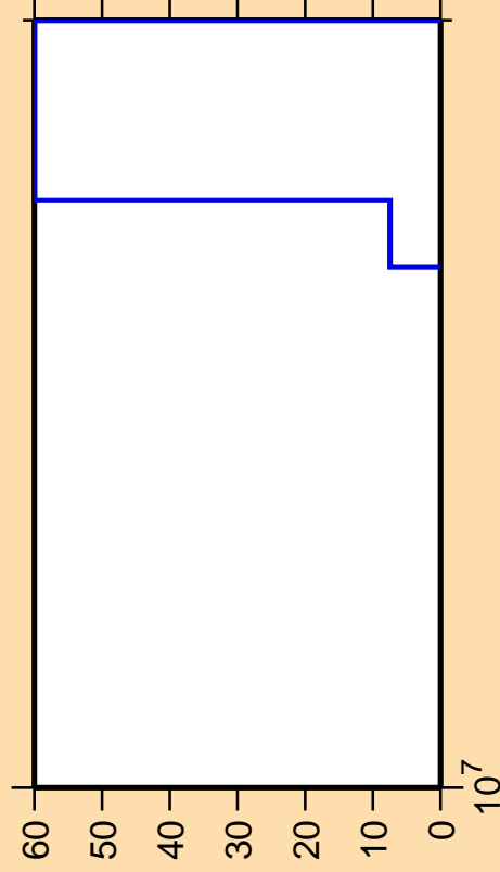
\Delta\sigma/\sigma vs. E for ^{193}\text{Hg}(\text{mt117})
