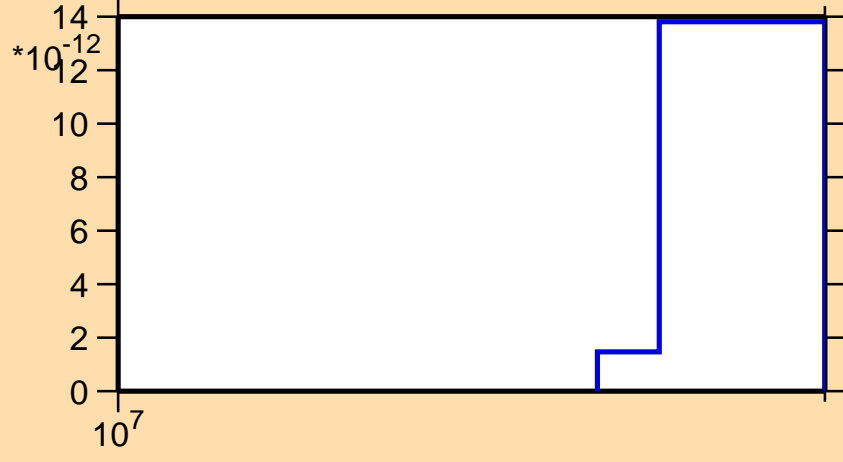
\sigma vs. E for ^{193}\text{Hg}(\text{mt117})
