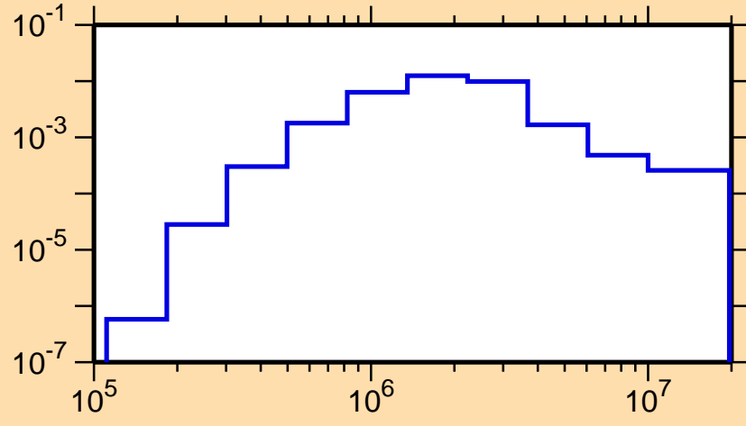
\sigma vs. E for ^{193}\text{Hg}(n,n_3)
