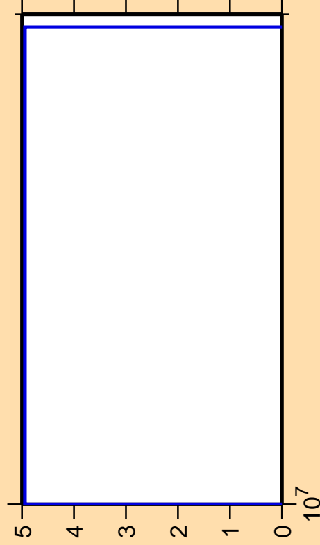
\Delta\sigma/\sigma vs. E for ^{193}\text{Hg}(n,nt)
