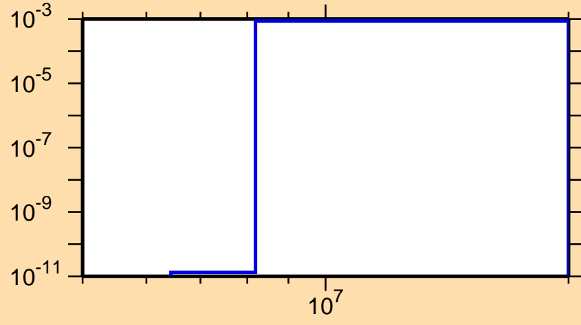
\sigma vs. E for ^{193}\text{Hg}(n,np)
