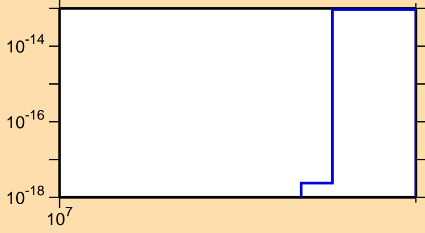
\sigma vs. E for ^{193}\text{Hg}(n,3n\alpha)
