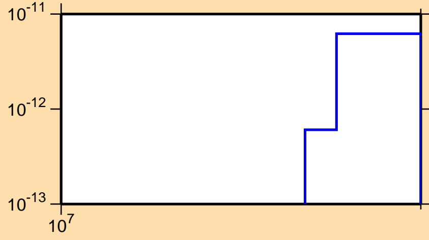
\sigma vs. E for ^{193}\text{Hg}(\text{mt117})
