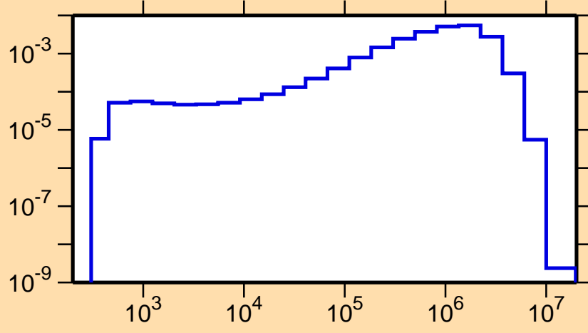
\sigma vs. E for ^{193}\text{Hg}(n,n_2)
