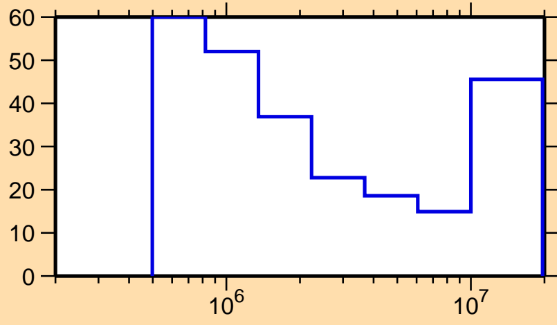
\Delta\sigma/\sigma vs. E for ^{193}\text{Hg}(n,n\text{cont.})
