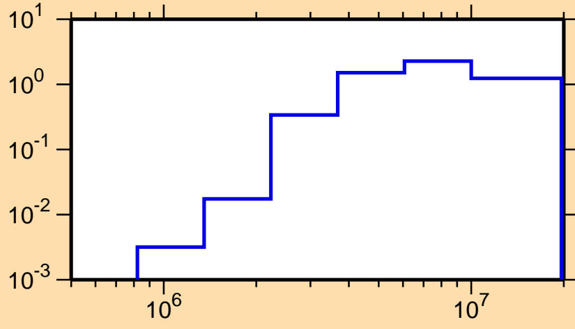
\sigma vs. E for ^{193}\text{Hg}(n,n\text{cont.})
