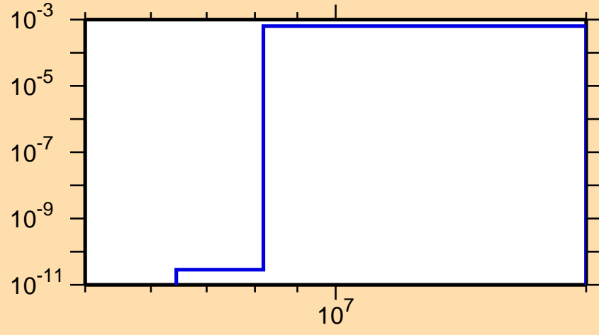
\sigma vs. E for ^{193}\text{Hg}(n,d)
