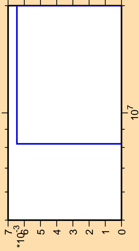
\Delta\sigma/\sigma vs. E for ^{193}\text{Hg}(n,3n\alpha)
