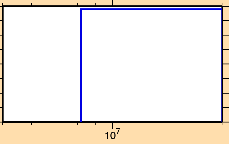
\sigma vs. E for ^{193}\text{Hg}(n,2np)
