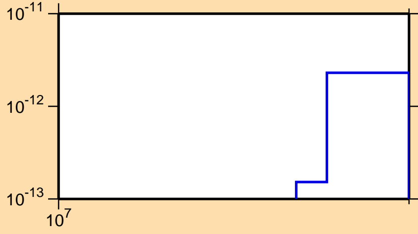
\sigma vs. E for ^{194}\text{Hg}(\text{mt117})
