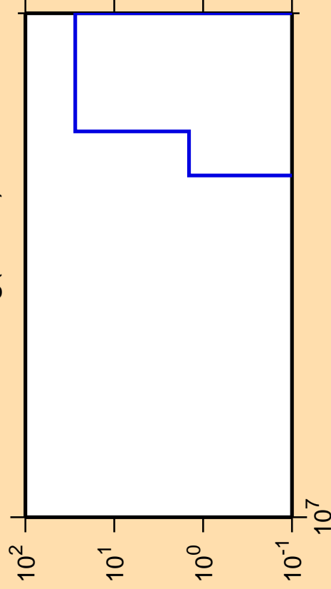
\Delta\sigma/\sigma vs. E for ^{194}\text{Hg} (mt 45)
