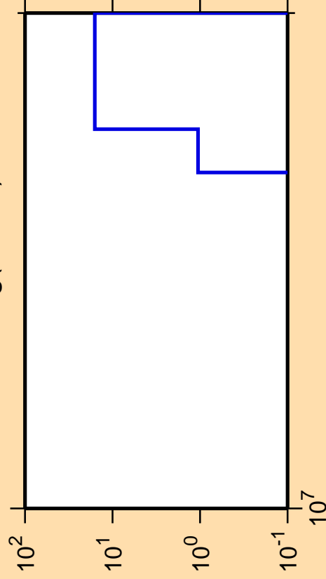
\Delta\sigma/\sigma vs. E for ^{194}\text{Hg}(\text{mt117})
