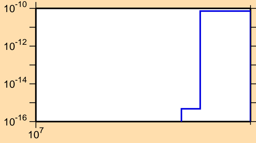
\sigma vs. E for ^{194}\text{Hg}(n,nt)
