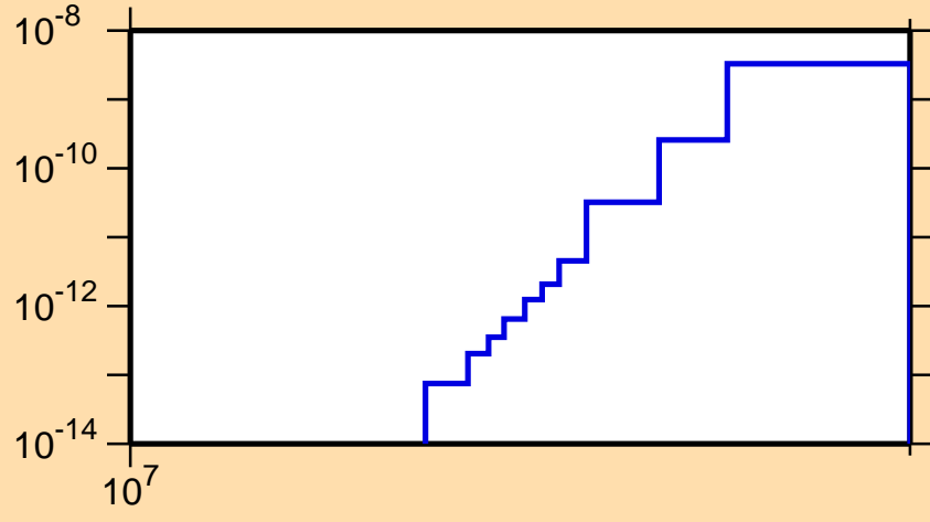
\sigma vs. E for ^{194}\text{Hg}(n,\text{He}3)
