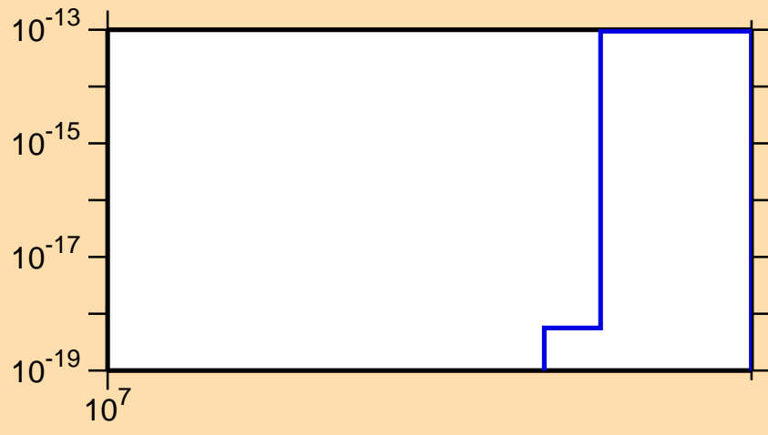
\sigma vs. E for ^{194}\text{Hg}(n,3n\alpha)
