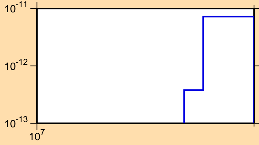
\sigma vs. E for ^{194}\text{Hg} (mt 45)
