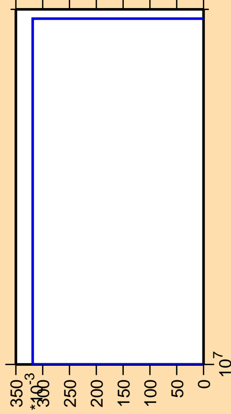
\Delta\sigma/\sigma vs. E for ^{194}\text{Hg} (mt 45)
