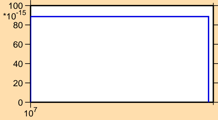
\sigma vs. E for ^{194}\text{Hg} (mt 45)
