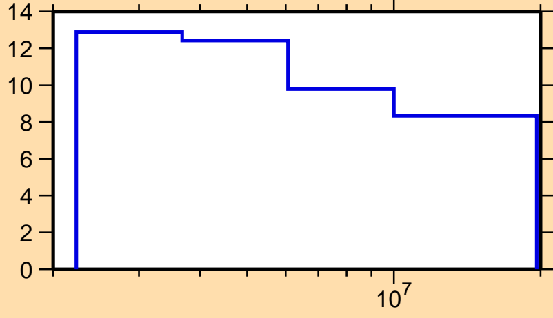
\Delta\sigma/\sigma vs. E for ^{194}\text{Hg}(n,n\text{onel.})
