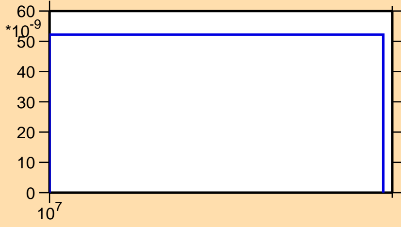
\sigma vs. E for ^{194}\text{Hg}(n,2n\alpha)
