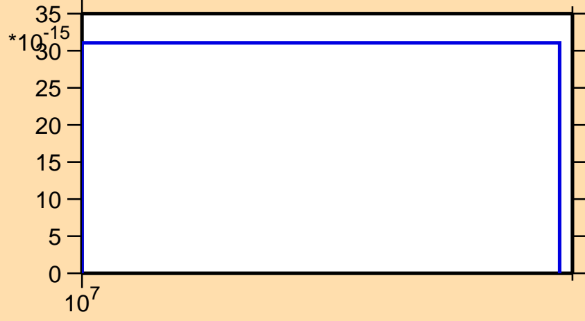
\sigma vs. E for ^{194}\text{Hg}(\text{mt117})
