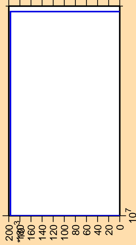
\Delta\sigma/\sigma vs. E for ^{194}\text{Hg}(\text{mt117})
