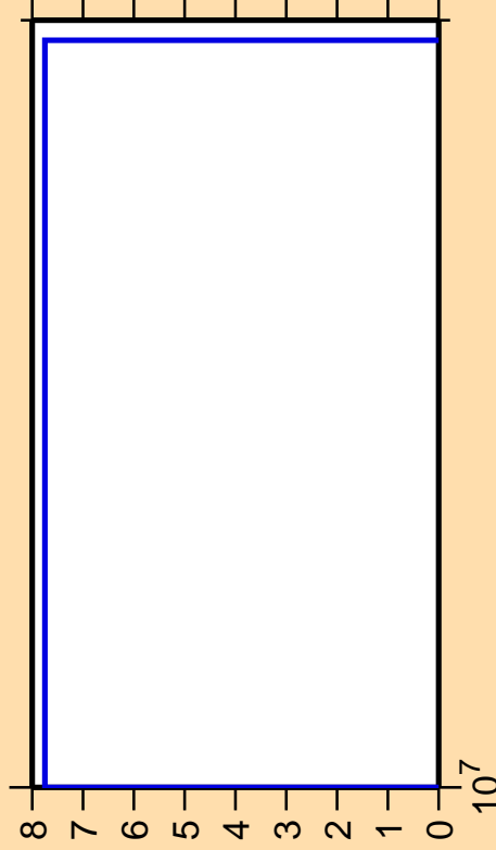
\Delta\sigma/\sigma vs. E for ^{195}\text{Hg}(n,nt)
