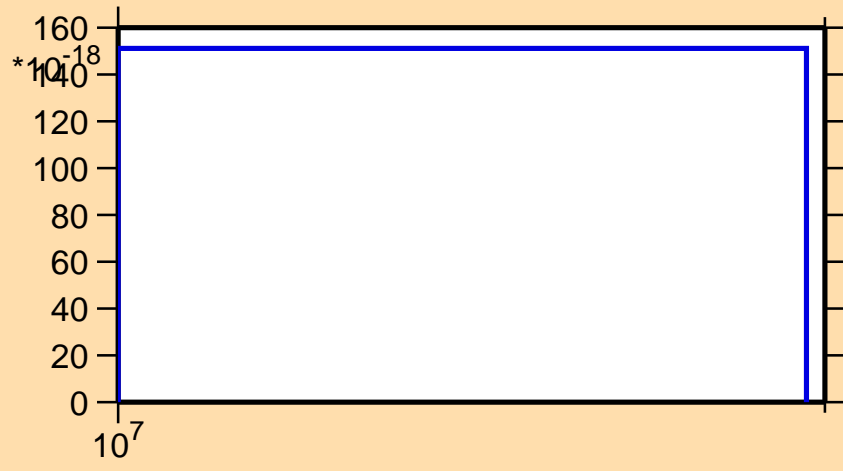
\sigma vs. E for ^{195}\text{Hg}(n,3n\alpha)
