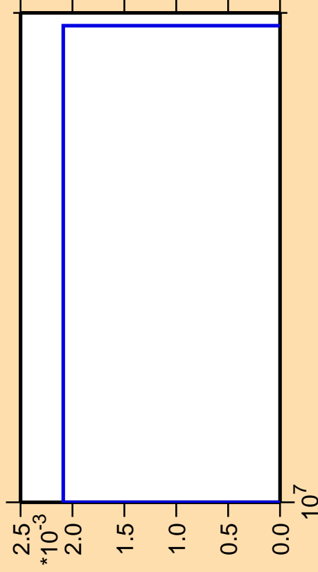
\Delta\sigma/\sigma vs. E for ^{195}\text{Hg} (mt 34)
