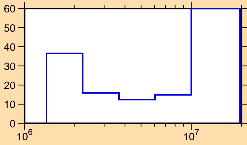
\Delta\sigma/\sigma vs. E for ^{195}\text{Hg}(n,n\text{cont.})
