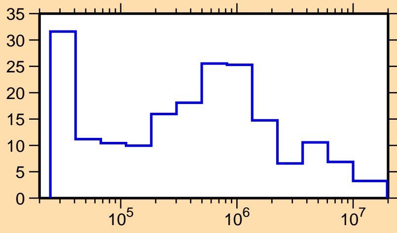
\Delta\sigma/\sigma vs. E for ^{195}\text{Hg}(n,\text{tot.})
