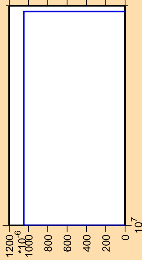
\Delta\sigma/\sigma vs. E for ^{195}\text{Hg}(n,3n\alpha)
