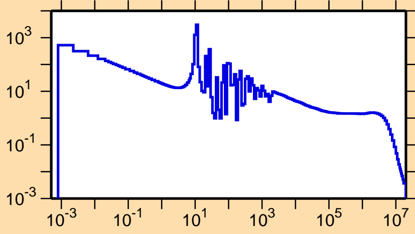
\sigma vs. E for ^{195}\text{Hg}(n,\gamma)
