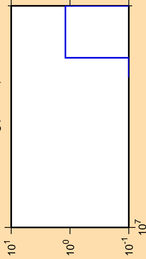
\Delta\sigma/\sigma vs. E for ^{195}\text{Hg}(\text{mt117})
