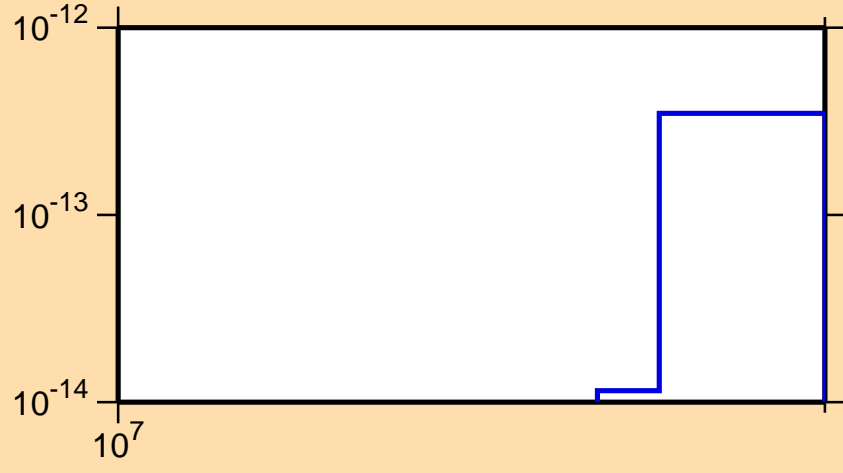
\sigma vs. E for ^{195}\text{Hg} (mt 45)
