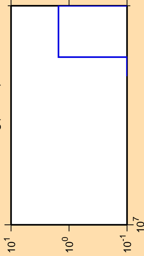
\Delta\sigma/\sigma vs. E for ^{195}\text{Hg} (mt 45)
