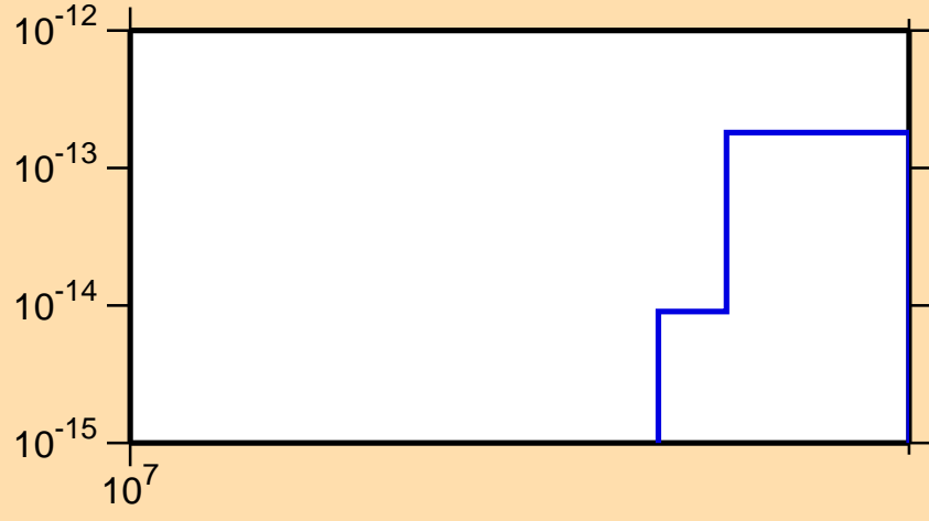
\sigma vs. E for ^{195}\text{Hg}(\text{mt117})
