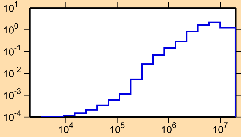
\sigma vs. E for ^{195}\text{Hg}(n,\text{inel.})
