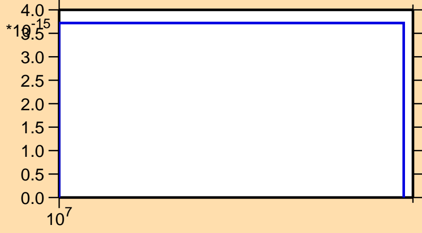
\sigma vs. E for ^{195}\text{Hg} (mt 45)
