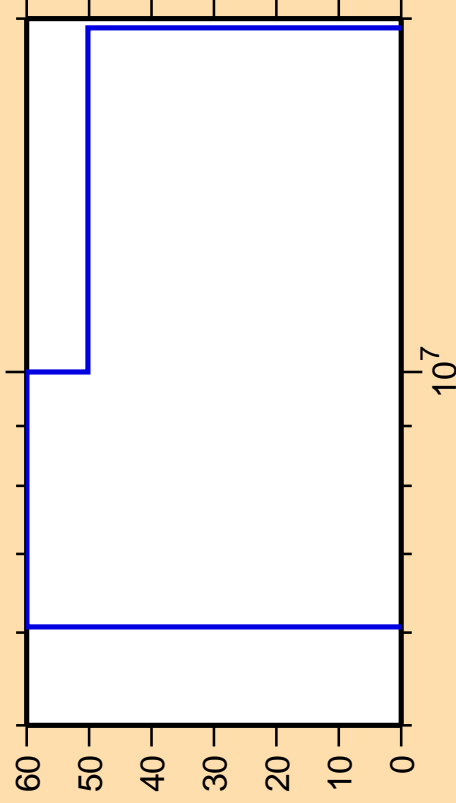
\Delta\sigma/\sigma vs. E for ^{195}\text{Hg}(n,np)
