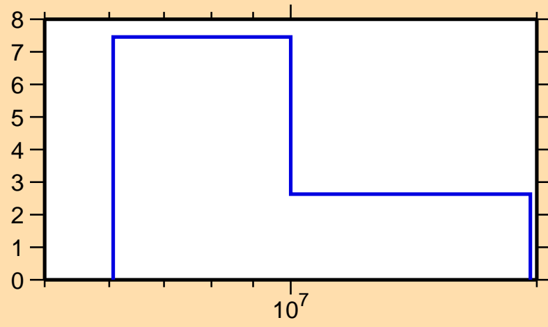
\Delta\sigma/\sigma vs. E for ^{195}\text{Hg}(n,\text{tot.})
