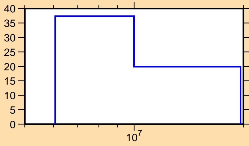
\Delta\sigma/\sigma vs. E for ^{195}\text{Hg}(n,2n)
