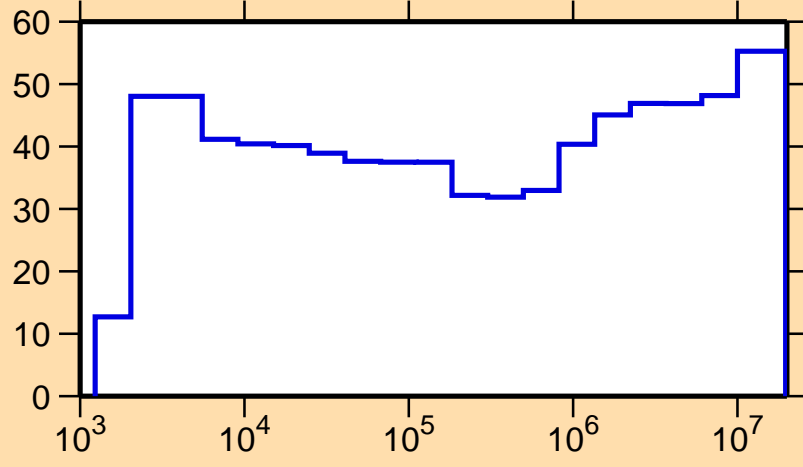
\Delta\sigma/\sigma vs. E for ^{195}\text{Hg}(n,n_1)
