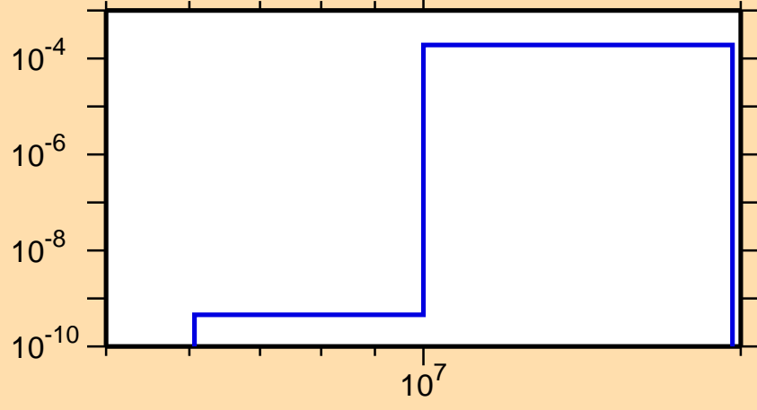
\sigma vs. E for ^{195}\text{Hg}(n,np)
