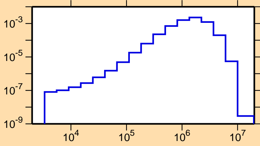
\sigma vs. E for ^{195}\text{Hg}(n,n_2)
