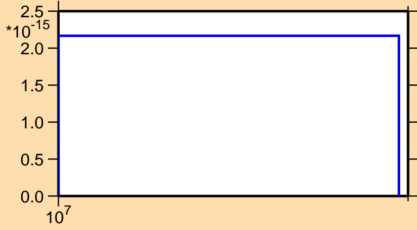
\sigma vs. E for ^{195}\text{Hg}(\text{mt117})
