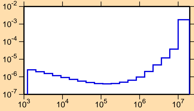
\sigma vs. E for ^{195}\text{Hg}(n,\alpha)
