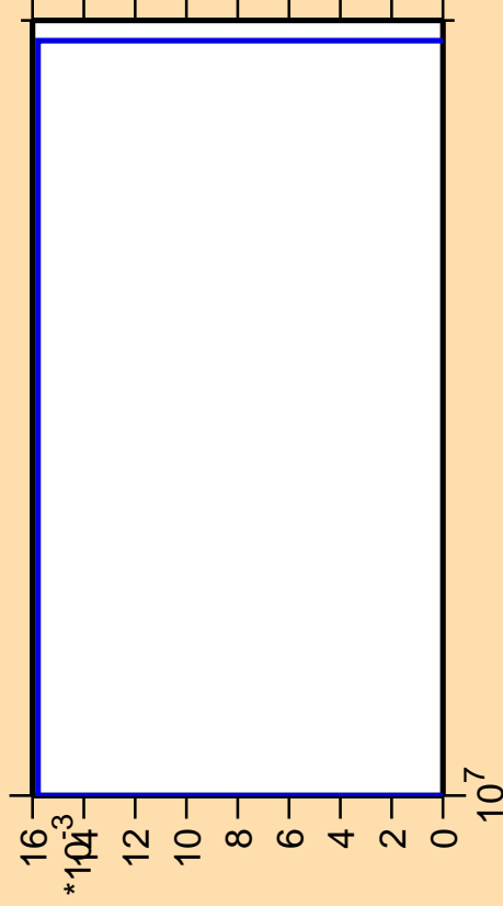
\Delta\sigma/\sigma vs. E for ^{195}\text{Hg} (mt 45)
