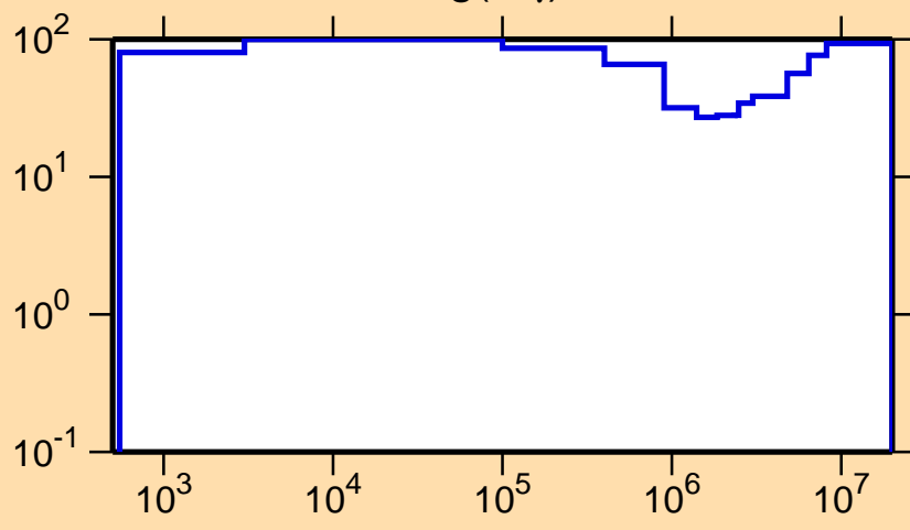
\Delta\sigma/\sigma vs. E for ^{195}\text{Hg}(n,\gamma)
