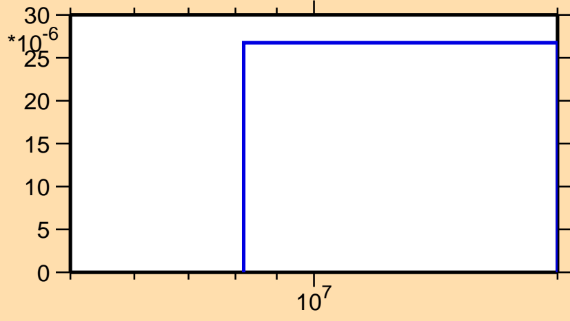
\sigma vs. E for ^{195}\text{Hg}(n,t)
