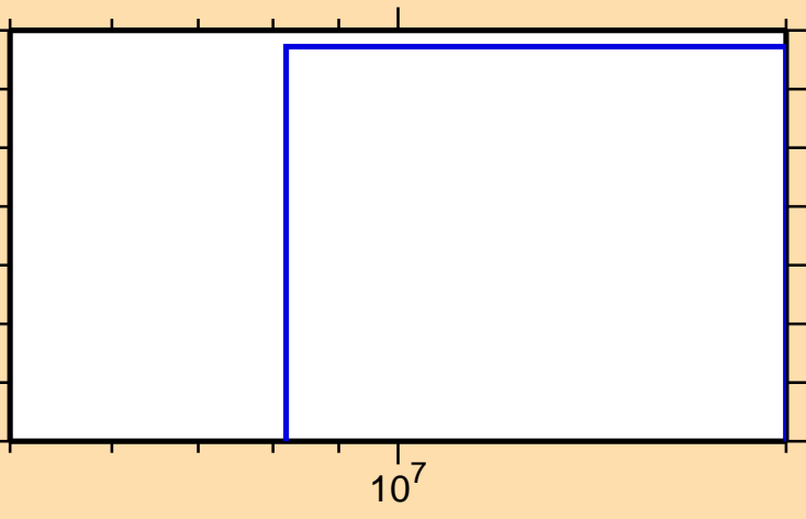
\sigma vs. E for ^{195}\text{Hg} (mt 45)
