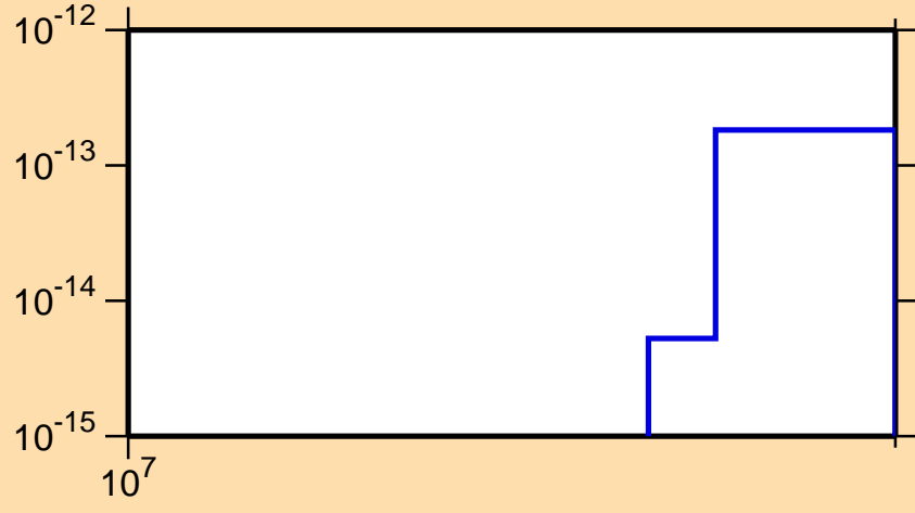
\sigma vs. E for ^{196}\text{Hg}(\text{mt117})
