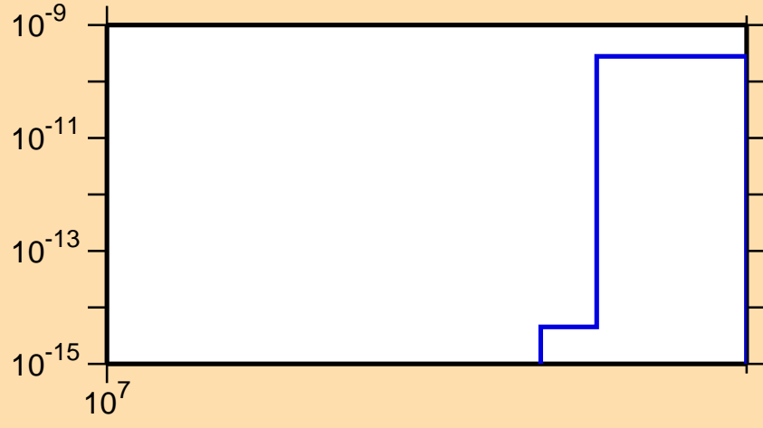
\sigma vs. E for ^{196}\text{Hg}(n,nt)
