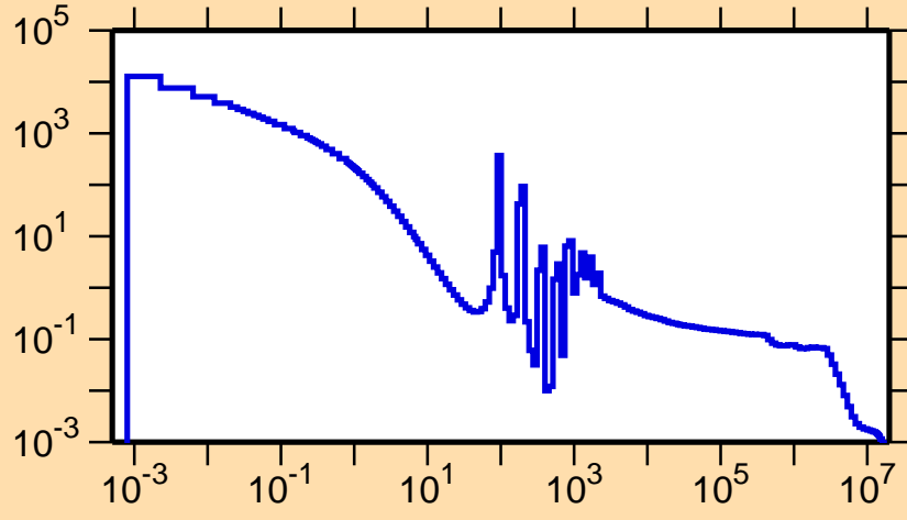
\sigma vs. E for ^{196}\text{Hg}(n,\gamma)
