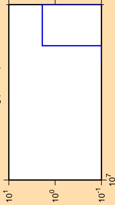
\Delta\sigma/\sigma vs. E for ^{196}\text{Hg} (mt 45)
