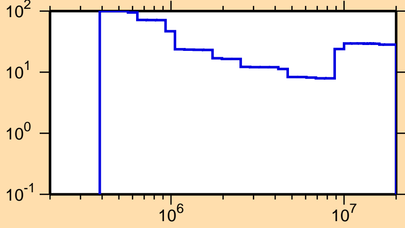
\Delta\sigma/\sigma vs. E for ^{196}\text{Hg}(n,\text{inel.})
