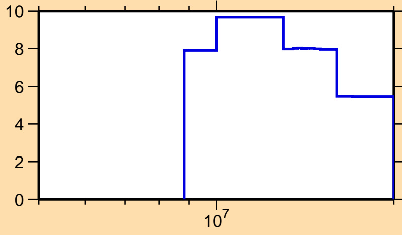
\Delta\sigma/\sigma vs. E for ^{196}\text{Hg}(n,\text{el.})
