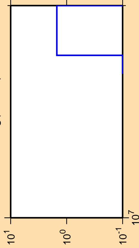
\Delta\sigma/\sigma vs. E for ^{196}\text{Hg}(\text{mt117})
