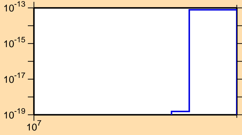
\sigma vs. E for ^{196}\text{Hg}(n,3n\alpha)
