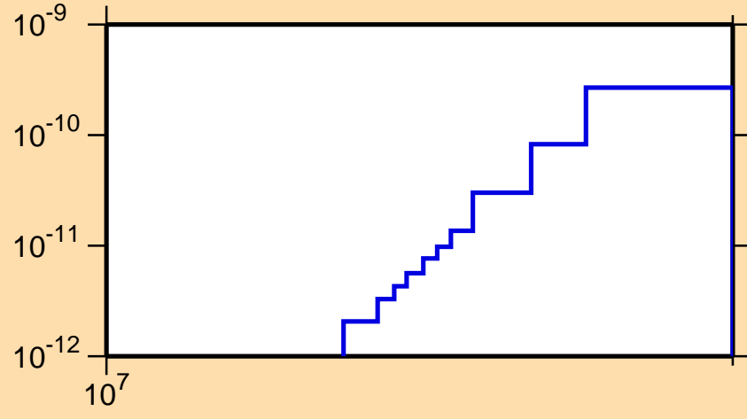
\sigma vs. E for ^{196}\text{Hg}(n,p\alpha)
