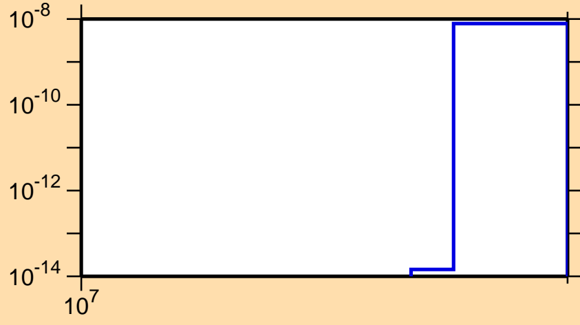
\sigma vs. E for ^{196}\text{Hg}(n,2np)
