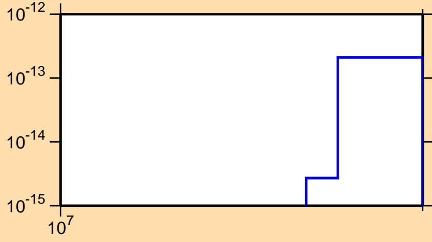
\sigma vs. E for ^{196}\text{Hg} (mt 45)
