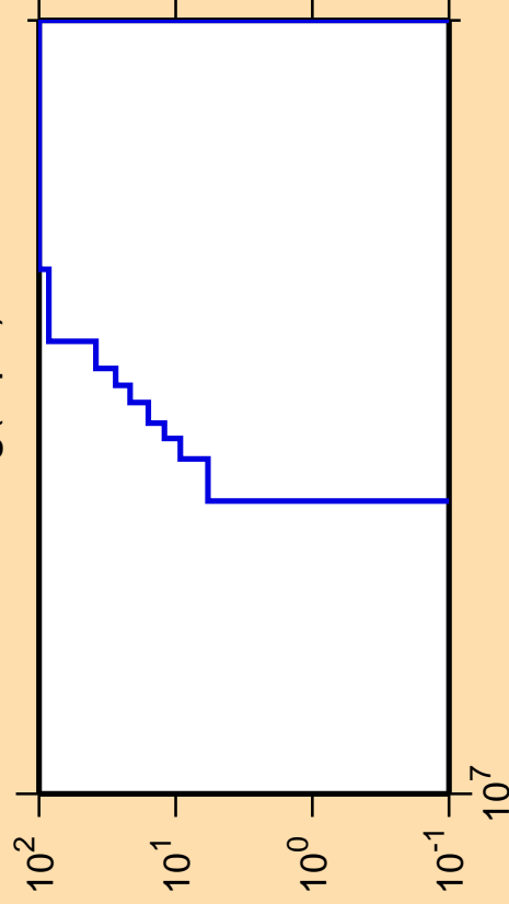
\Delta\sigma/\sigma vs. E for ^{196}\text{Hg}(n,p\alpha)
