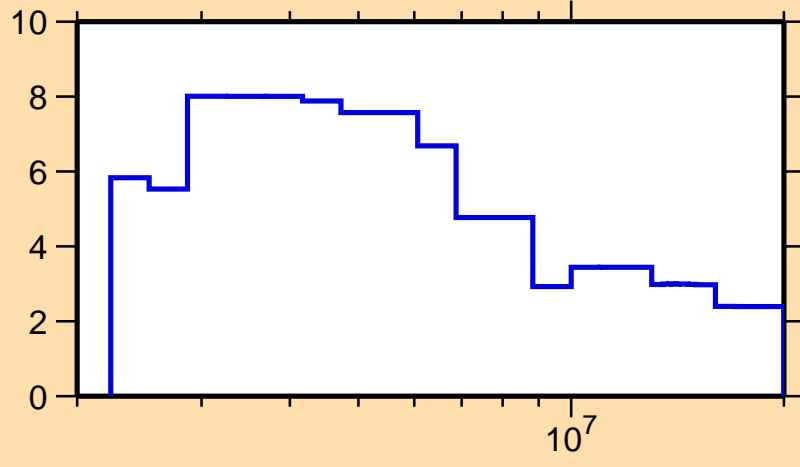
\Delta\sigma/\sigma vs. E for ^{196}\text{Hg}(n,\text{tot.})
