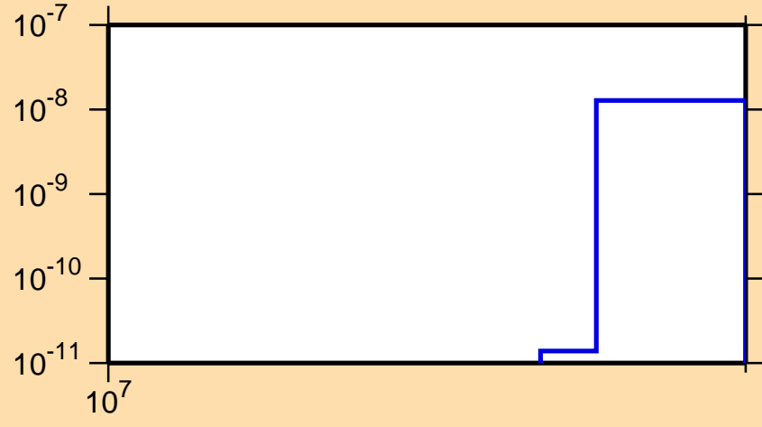
\sigma vs. E for ^{196}\text{Hg}(n,\text{nd})
