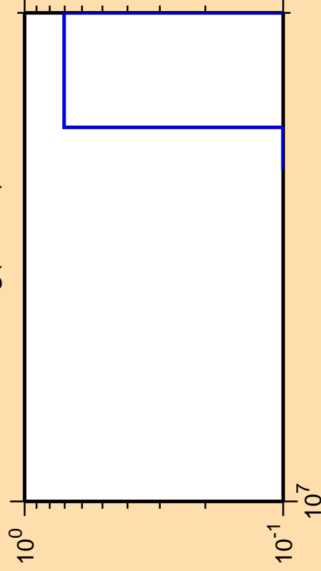
\Delta\sigma/\sigma vs. E for ^{196}\text{Hg}(n,3n\alpha)
