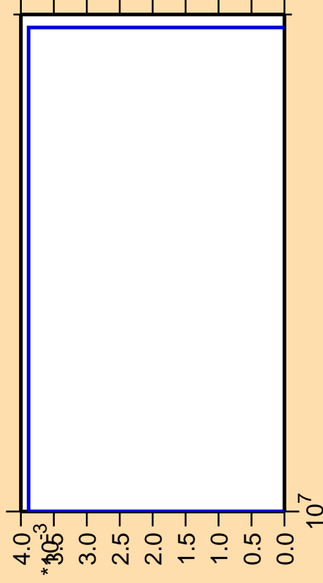
\Delta\sigma/\sigma vs. E for ^{196}\text{Hg}(n,3n\alpha)
