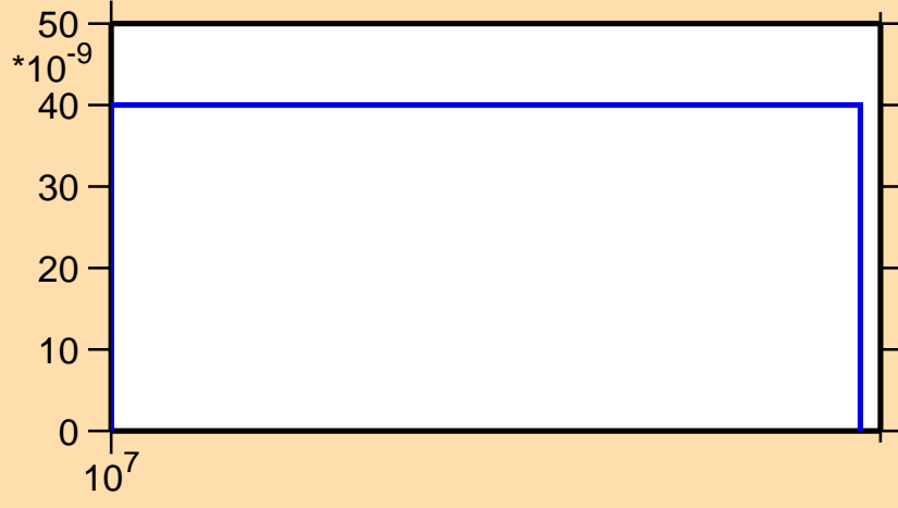
\sigma vs. E for ^{196}\text{Hg}(n,2n\alpha)
