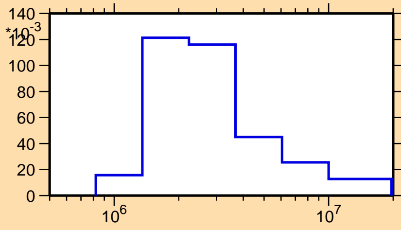
\sigma vs. E for ^{196}\text{Hg}(n,n_4)
