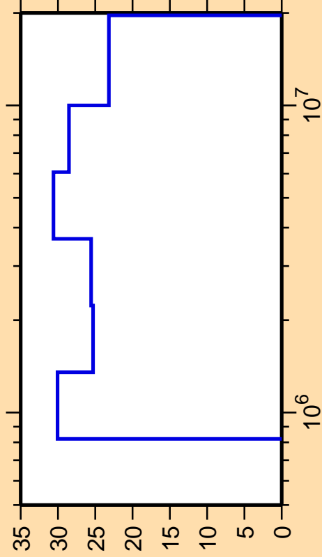
\Delta\sigma/\sigma vs. E for ^{196}\text{Hg}(n,n_4)
