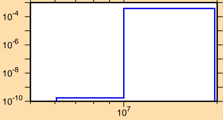
\sigma vs. E for ^{196}\text{Hg}(n,np)
