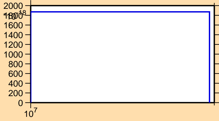
\sigma vs. E for ^{196}\text{Hg}(\text{mt117})
