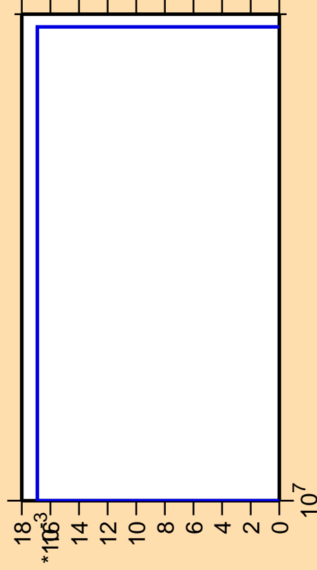
\Delta\sigma/\sigma vs. E for ^{196}\text{Hg} (mt 45)
