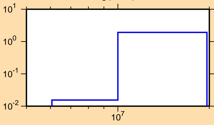
\sigma vs. E for ^{196}\text{Hg}(n,2n)
