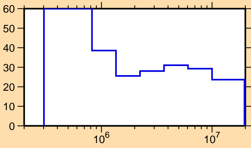
\Delta\sigma/\sigma vs. E for ^{196}\text{Hg}(n,n_1)
