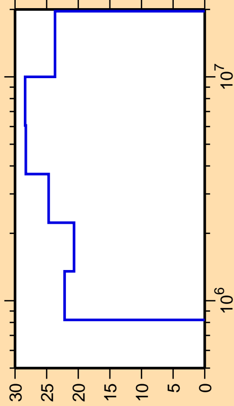
\Delta\sigma/\sigma vs. E for ^{196}\text{Hg}(n,n_3)
