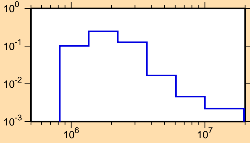
\sigma vs. E for ^{196}\text{Hg}(n,n_2)
