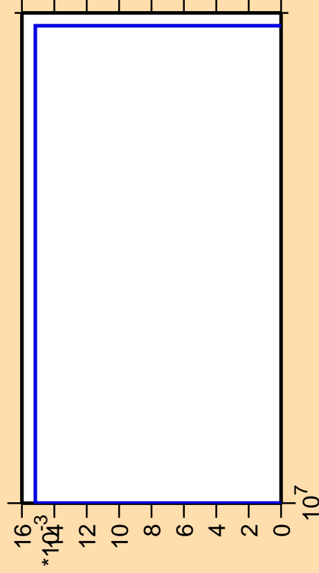
\Delta\sigma/\sigma vs. E for ^{196}\text{Hg}(\text{mt117})
