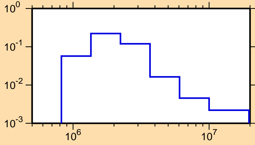
\sigma vs. E for ^{196}\text{Hg}(n,n_3)
