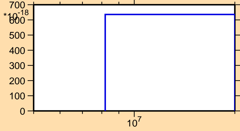
\sigma vs. E for ^{196}\text{Hg}(n,3n\alpha)
