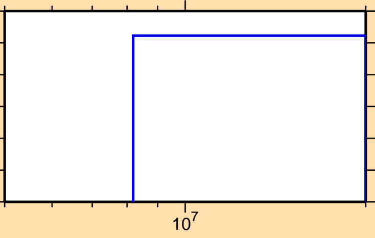
\sigma vs. E for ^{196}\text{Hg}(n,\text{nd})
