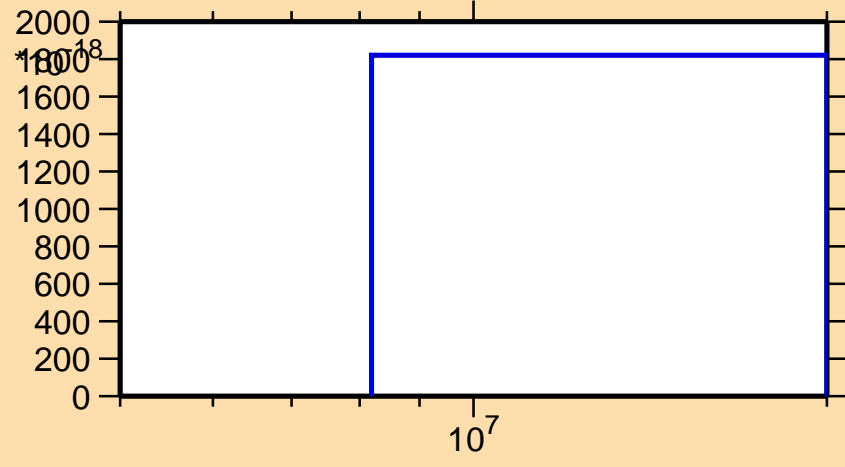
\sigma vs. E for ^{196}\text{Hg} (mt 45)
