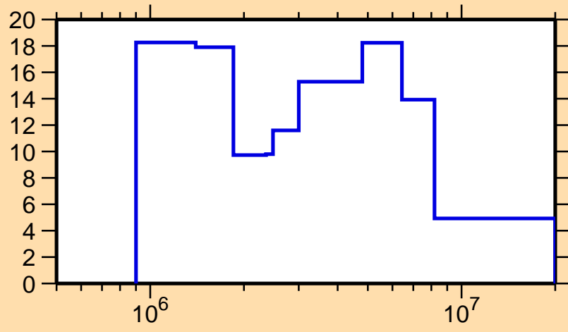
\Delta\sigma/\sigma vs. E for ^{197}\text{Hg}(n,el.)
