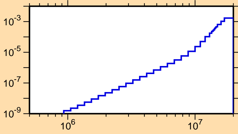
\sigma vs. E for ^{198}\text{Hg}(n,\alpha)
