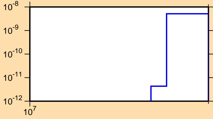
\sigma vs. E for ^{198}\text{Hg}(n,\text{nd})
