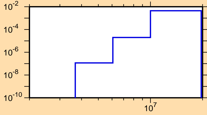
\sigma vs. E for ^{198}\text{Hg}(n,p)
