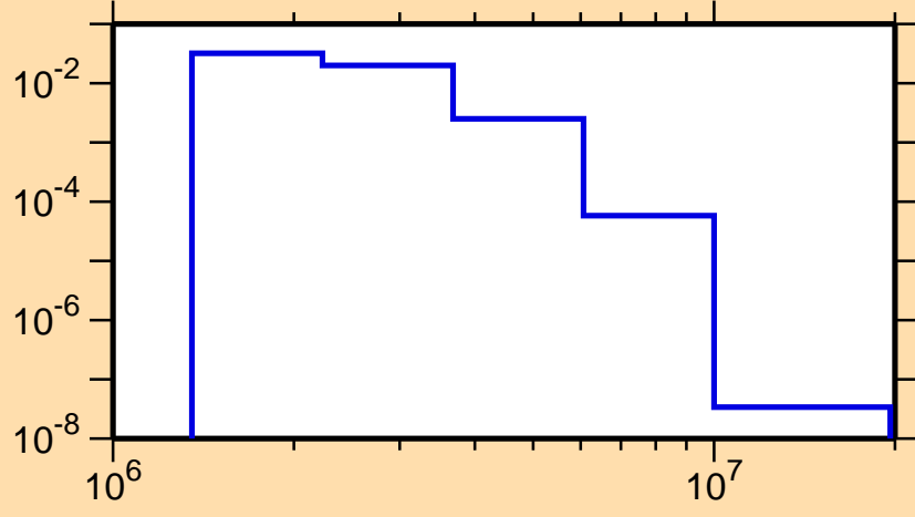
\sigma vs. E for ^{198}\text{Hg}(n,n_4)
