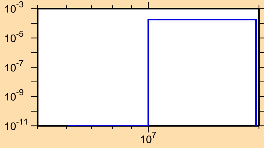
\sigma vs. E for ^{198}\text{Hg}(n,d)
