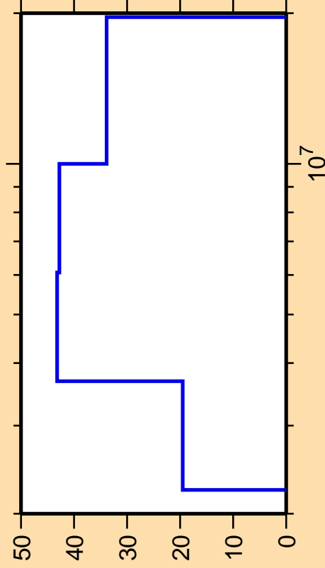
\Delta\sigma/\sigma vs. E for ^{198}\text{Hg}(n,p)
