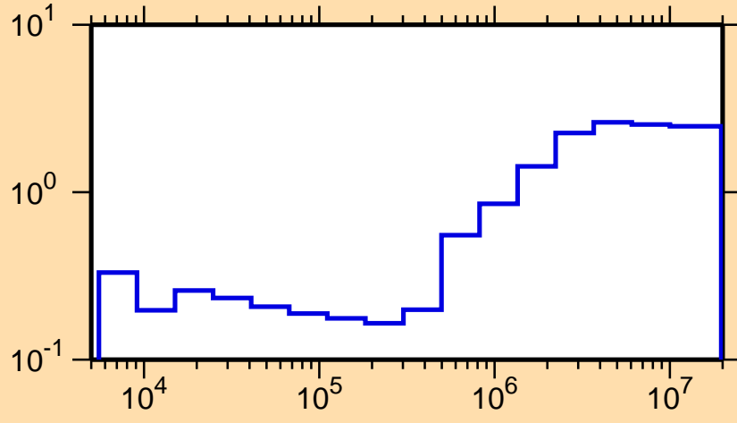
\sigma vs. E for ^{198}\text{Hg}(n,\text{nonel.})
