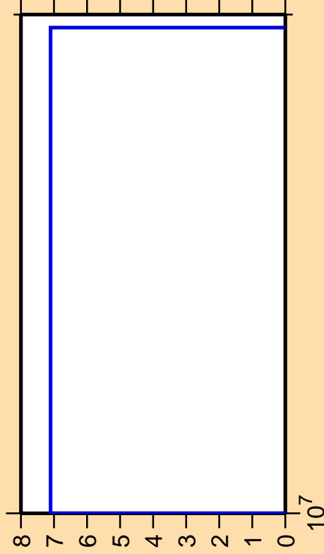
\Delta\sigma/\sigma vs. E for ^{198}\text{Hg}(n,nt)
