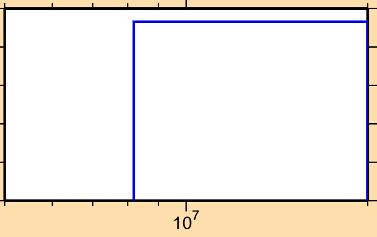
\sigma vs. E for ^{198}\text{Hg}(n,p\alpha)
