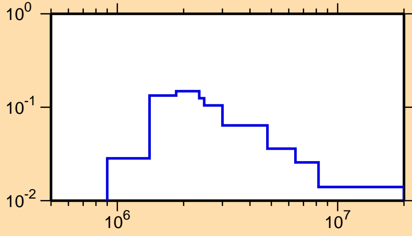
\sigma vs. E for ^{198}\text{Hg}(n,n_2)
