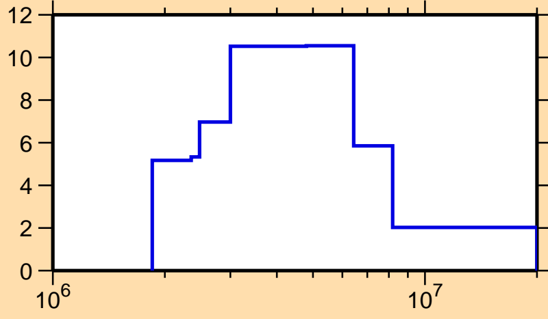
\Delta\sigma/\sigma vs. E for ^{198}\text{Hg}(n,\text{tot.})
