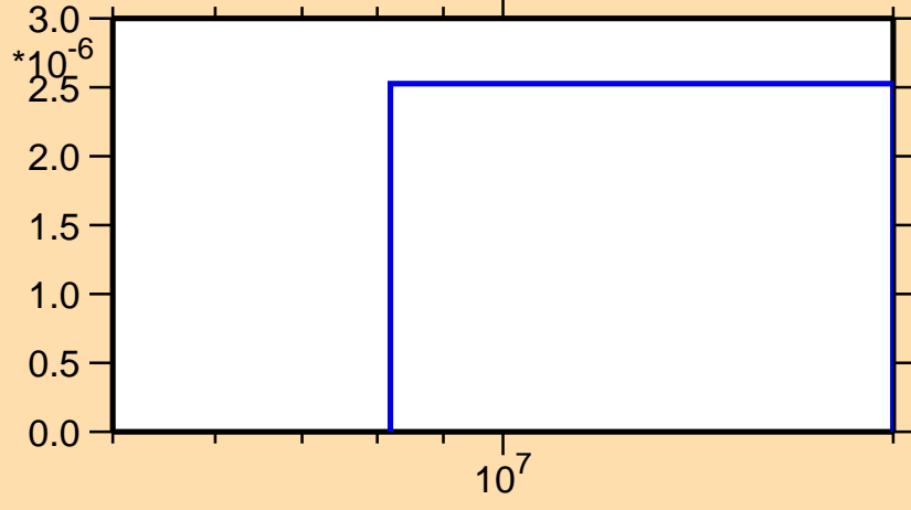
\sigma vs. E for ^{198}\text{Hg}(n,t)
