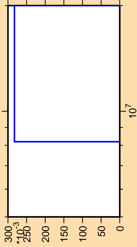
\Delta\sigma/\sigma vs. E for ^{198}\text{Hg}(n,p\alpha)
