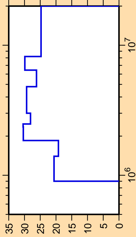
\Delta\sigma/\sigma vs. E for ^{198}\text{Hg}(n,n_2)
