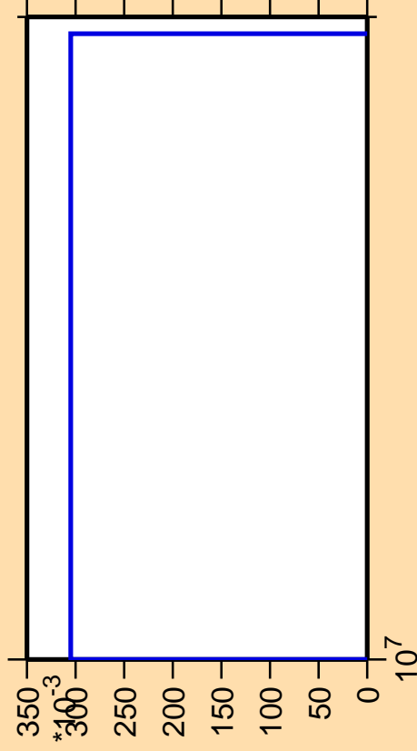
\Delta\sigma/\sigma vs. E for ^{199}\text{Hg}(n,p\alpha)
