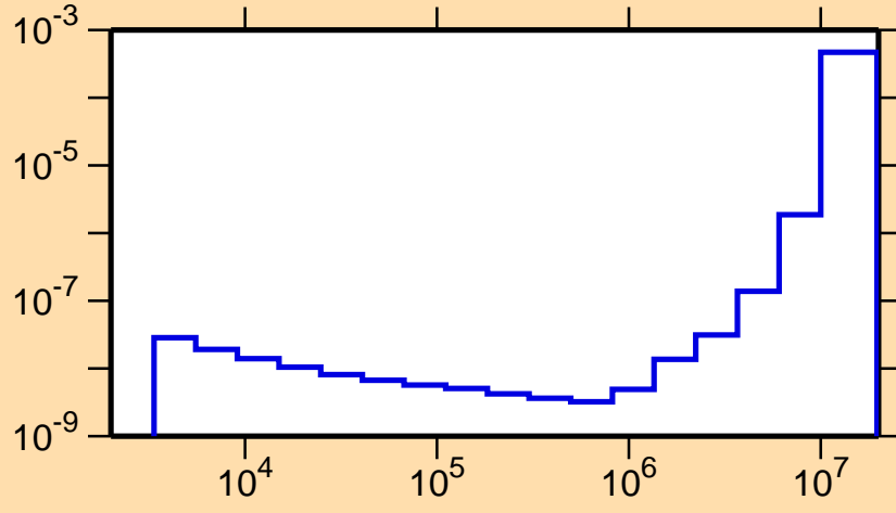
\sigma vs. E for ^{199}\text{Hg}(n,\alpha)
