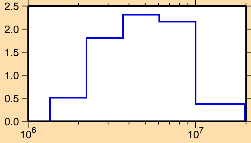
\sigma vs. E for ^{199}\text{Hg}(n,n\text{cont.})
