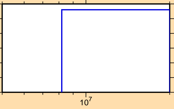
\sigma vs. E for ^{199}\text{Hg}(n,np)
