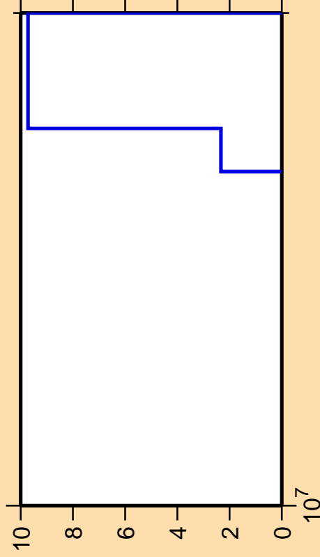
\Delta\sigma/\sigma vs. E for ^{199}\text{Hg}(n,p\alpha)
