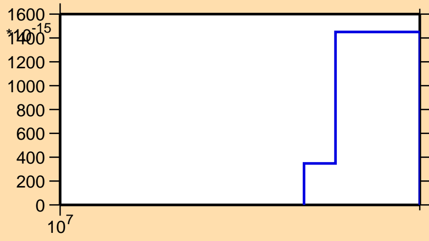
\sigma vs. E for ^{199}\text{Hg}(n,p\alpha)
