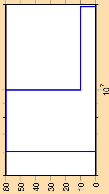
\Delta\sigma/\sigma vs. E for ^{199}\text{Hg}(n,2n)
