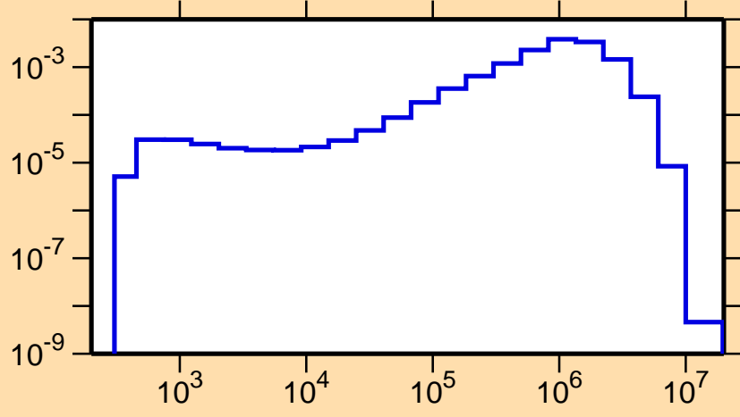
\sigma vs. E for ^{199}\text{Hg}(n,n_3)
