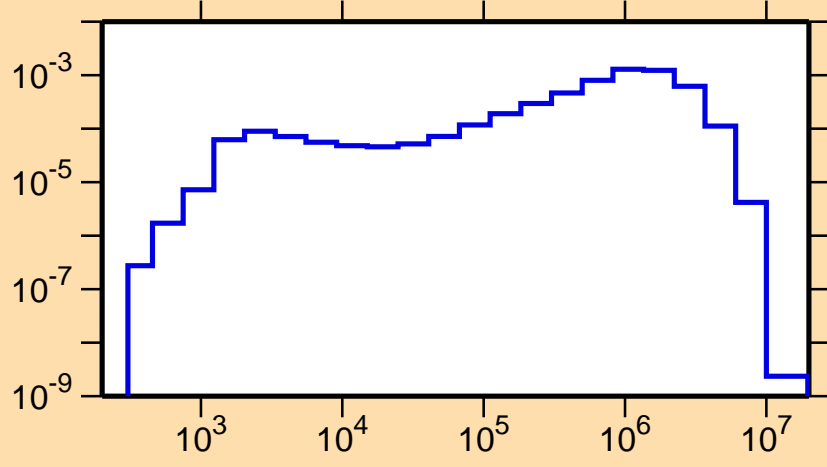
\sigma vs. E for ^{199}\text{Hg}(n,n_1)
