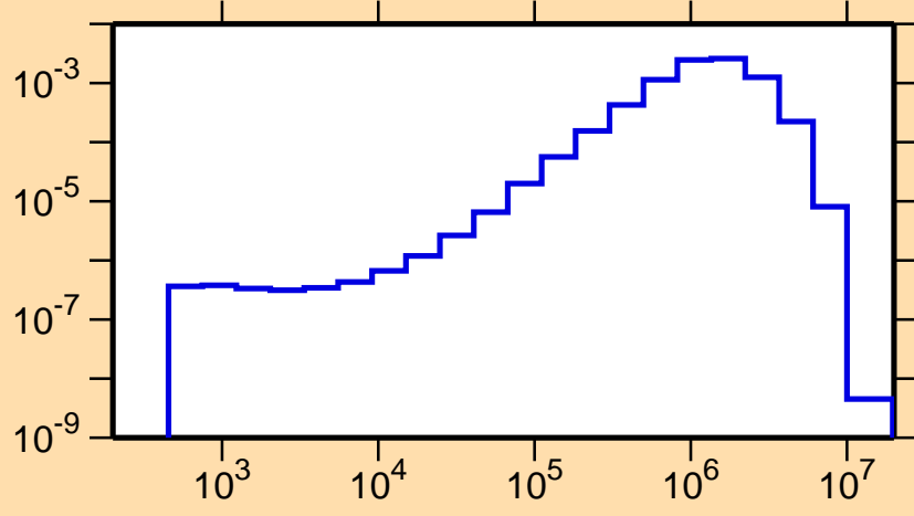
\sigma vs. E for ^{199}\text{Hg}(n,n_4)
