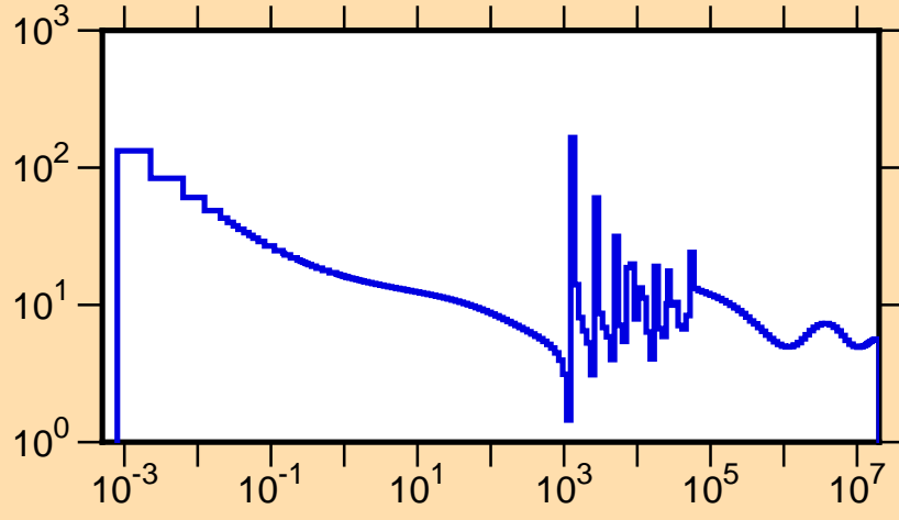
\sigma vs. E for ^{200}\text{Hg}(n,\text{tot.})
