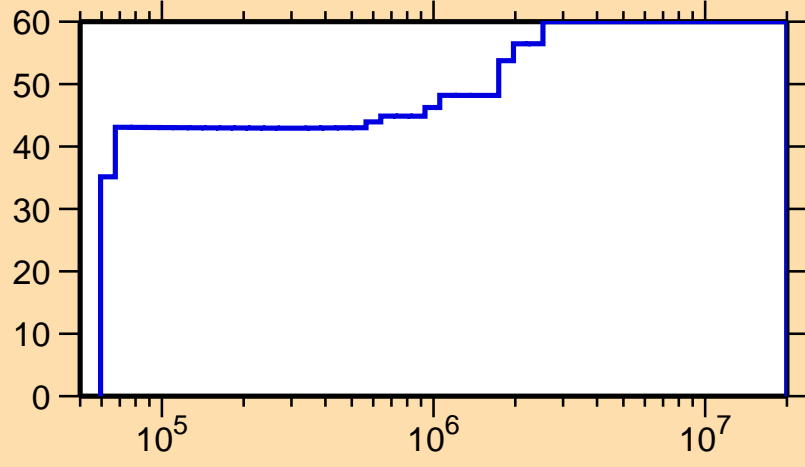
\Delta\sigma/\sigma vs. E for ^{200}\text{Hg}(n,\gamma)
