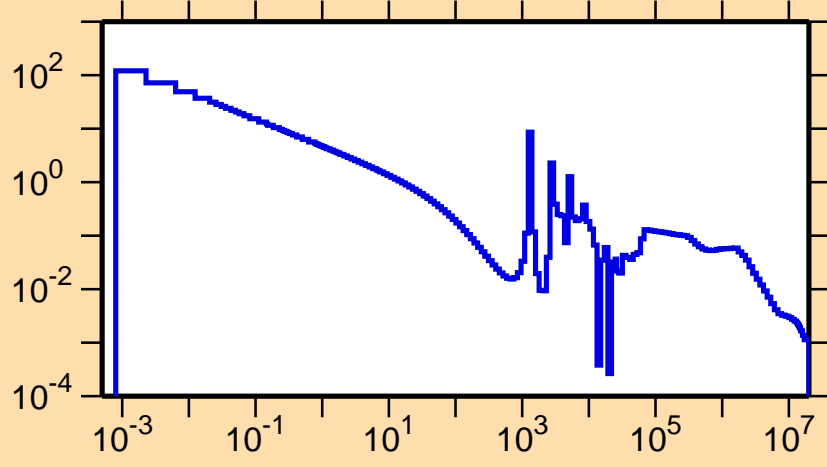
\sigma vs. E for ^{200}\text{Hg}(n,\gamma)
