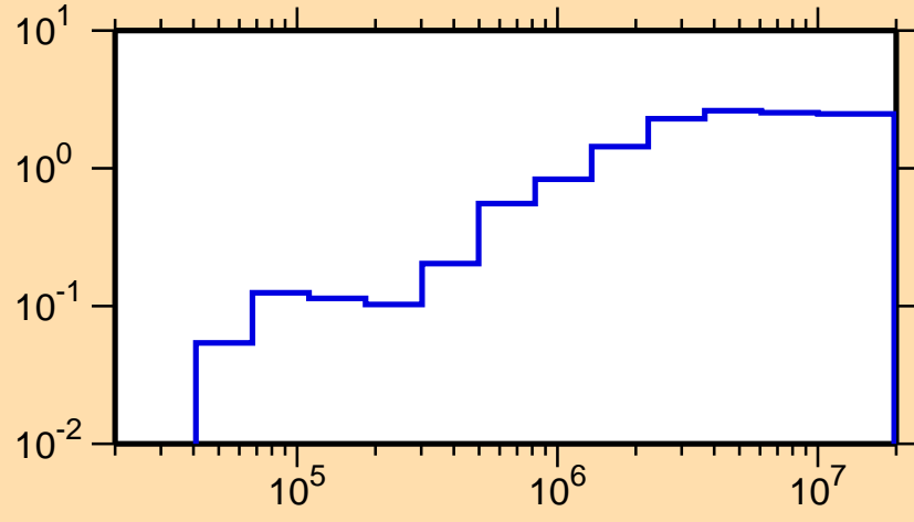
\sigma vs. E for ^{200}\text{Hg}(n,\text{nonel.})
