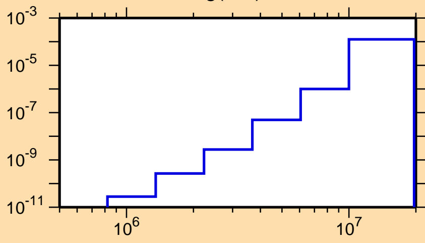
\sigma vs. E for ^{200}\text{Hg}(n,\alpha)
