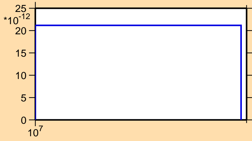
\sigma vs. E for ^{200}\text{Hg}(n,\text{nd})
