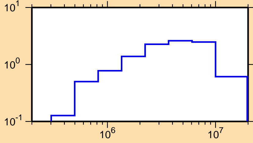
\sigma vs. E for ^{200}\text{Hg}(n,\text{inel.})
