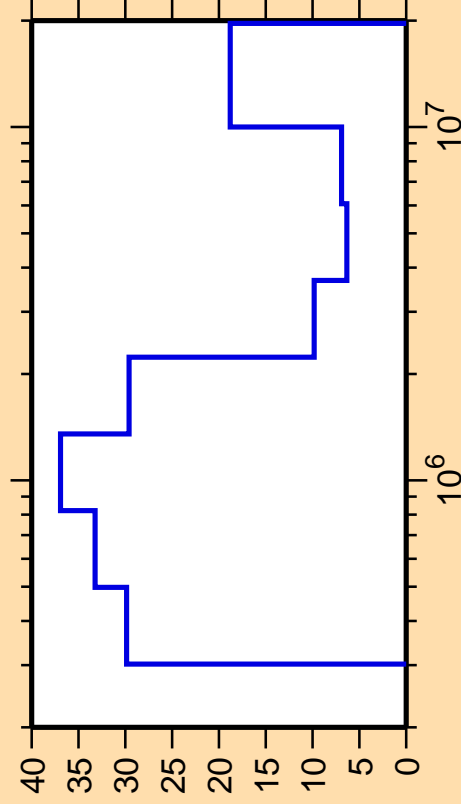
\Delta\sigma/\sigma vs. E for ^{200}\text{Hg}(n,\text{inel.})
