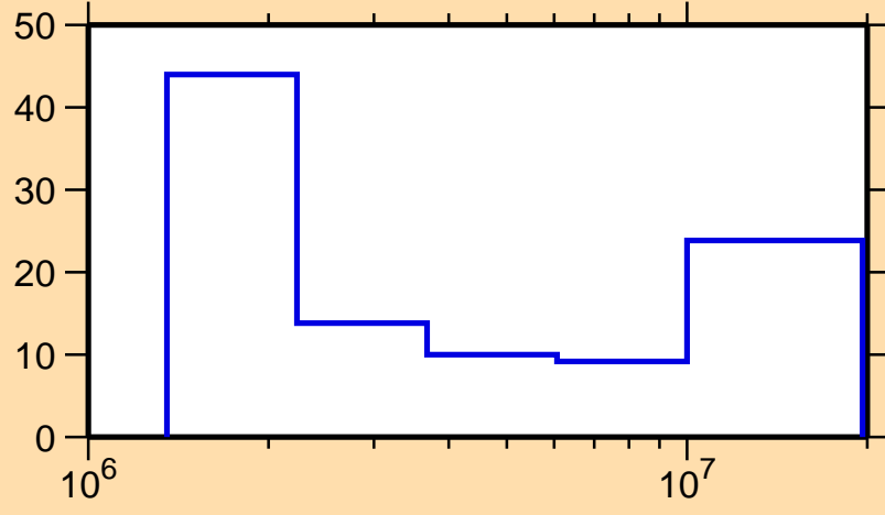
\Delta\sigma/\sigma vs. E for ^{200}\text{Hg}(n,n\text{cont.})
