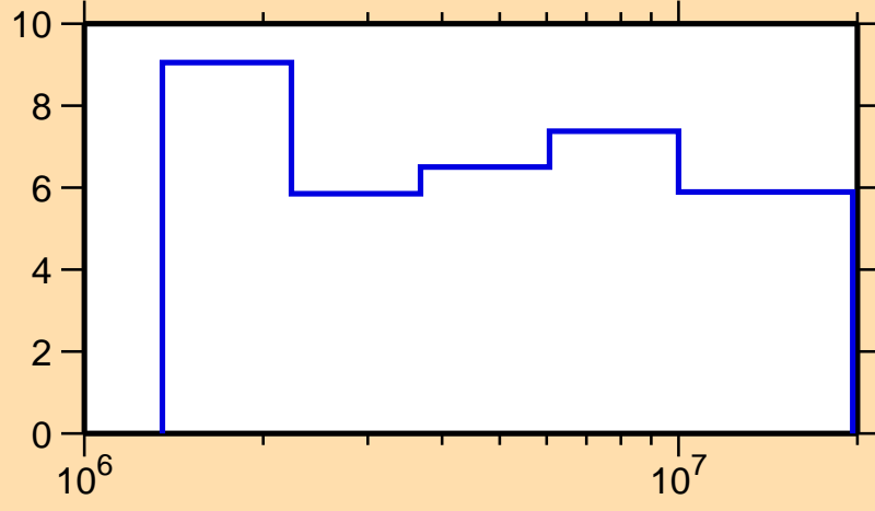
\Delta\sigma/\sigma vs. E for ^{200}\text{Hg}(n, el.)
