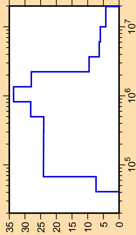
\Delta\sigma/\sigma vs. E for ^{200}\text{Hg}(n,\text{nonel.})
